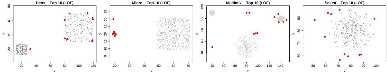
Figure 3.8: Synthetic data: LOF ( MinPts = 10 to 30 , top 10 ).
