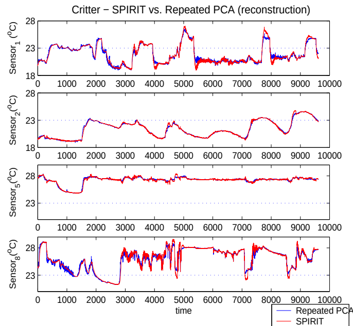
Figure 13.6: Reconstructions \tilde{\mathbf{x}}_t for Crittler. Repeated PCA requires (i) storing the entire data and (ii) performing PCA at each time tick (quadratic time, at best—for example, wall clock times here are 1.5 minutes versus 7 seconds).
