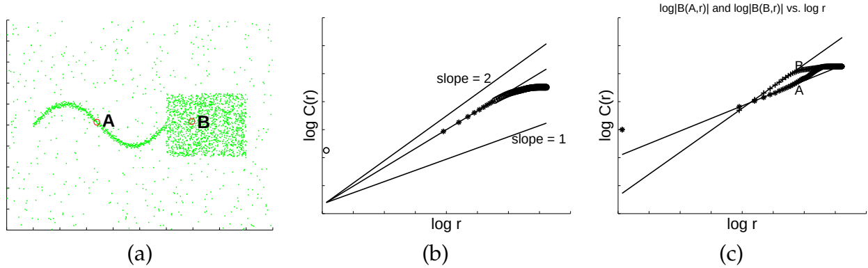
Figure 5.3: A dataset that contains two subsets of different intrinsic dimensionality
