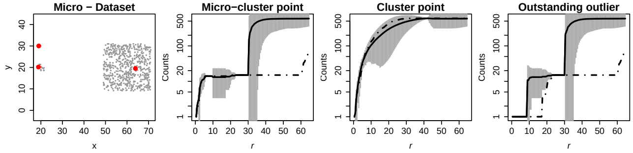
Figure 3.4: LOCI plots from an actual dataset—see also Section 3.5.
