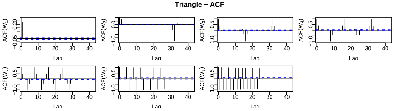
Figure 12.18: ACF (per DWT level) for Triangle.
