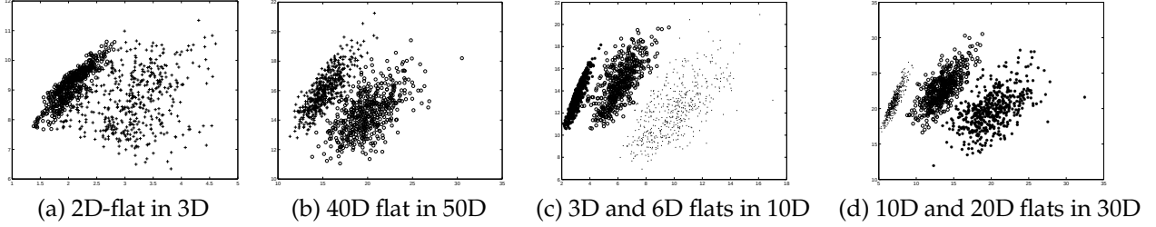
Figure 5.7: Discovering m -flats with DIC
