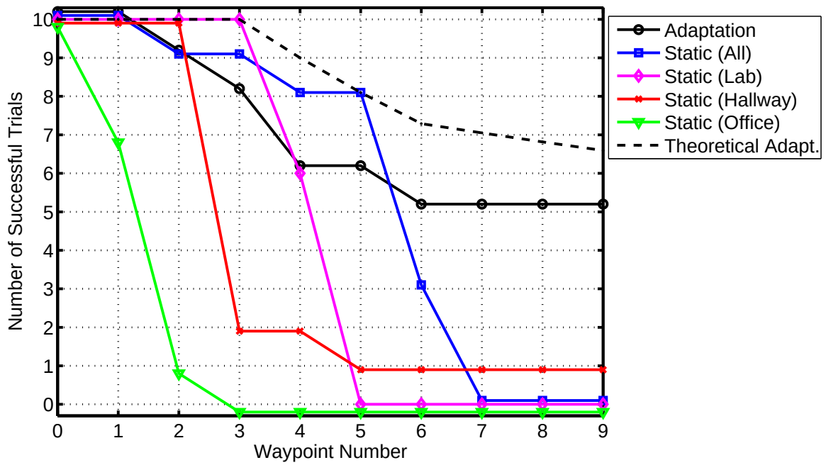
Figure 6.15: Results from the ball chasing task in the forward direction. The x axis shows the waypoint number. The y axis counts the successes in reaching this waypoint out of 10 runs.
