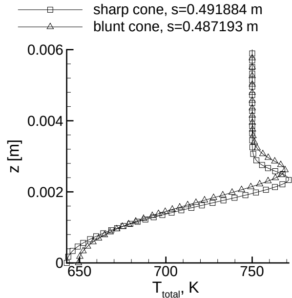
Figure 6: TLNS Total Temperature Profiles for Stetson Sharp and Blunt Cones at Blunt-Cone Flow Conditions, from Kufner via Hein
