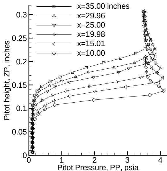
Figure 3: Mean Pitot Profiles for Stetson Sharp Cone
