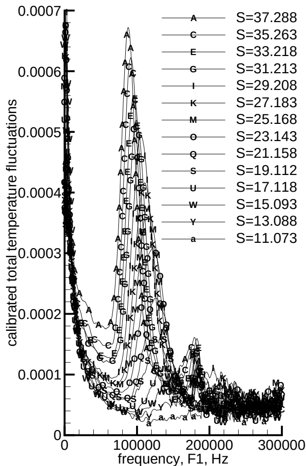
Figure 9: Total-Temperature Spectra for Stetson Sharp Cone
