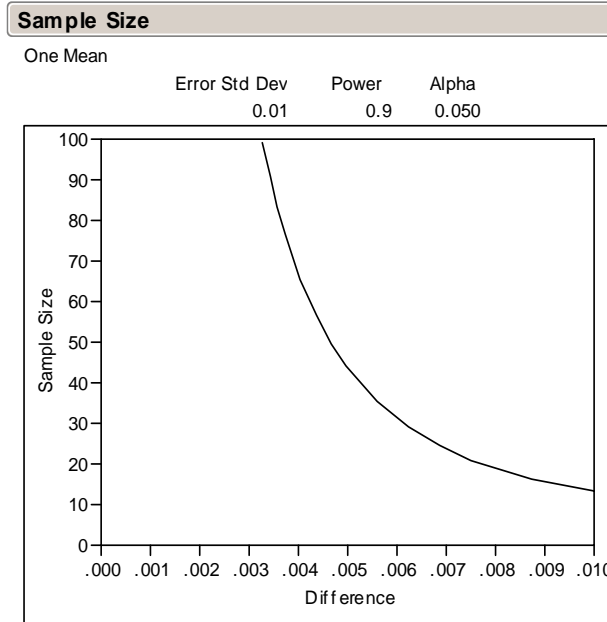
Figure 11. 0.9 Power Curve
