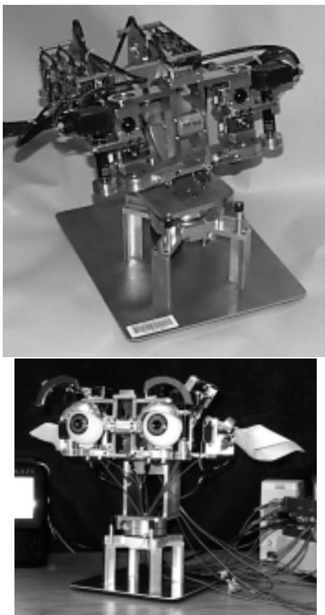
Figure 2: We have built two active vision heads, similar in design to Cog's head. On top is a desktop version with a 1 DOF neck, and below a head with actuators to include facial expressions.
