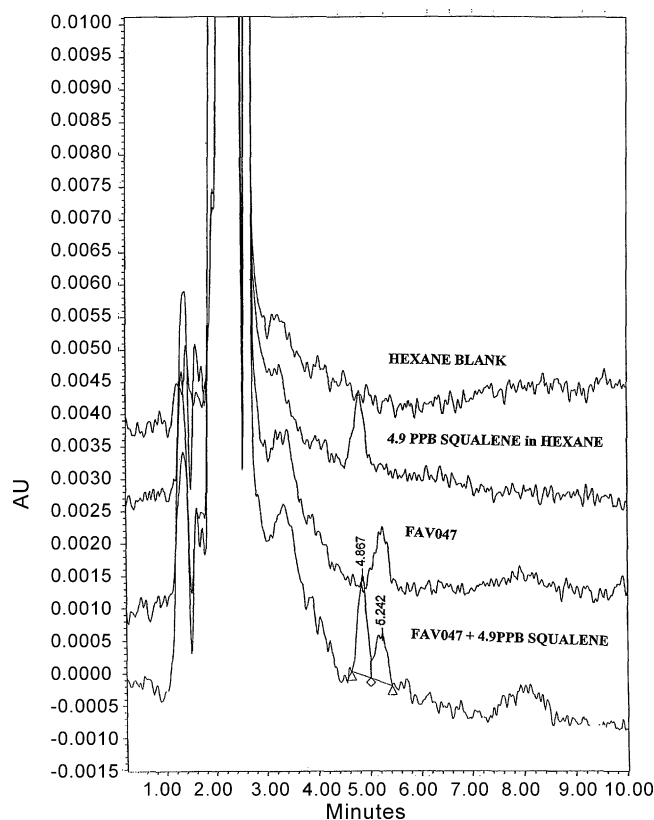
Fig. 4. Overlaid chromatograms for the hexane blank, squalene at 4.9 \mu\text{g l}^{-1} (ppb), Lot FAV047, and Lot FAV047 spiked with squalene at 4.9 \mu\text{g l}^{-1} (ppb).
