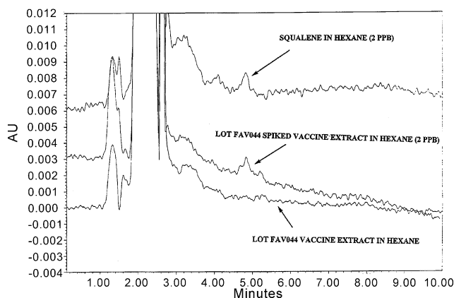
Fig. 2. Chromatograms of squalene in 2-propanol/hexane and in a hexane extract of spiked vaccine (Lot FAV044) at this limit of detection.
