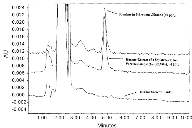
Fig. 1. Overlay chromatographic profiles of squalene in 2-propanol/hexane (40 ppb), hexane extract from a 40-ppb squalene-spiked Lot FAV044, and hexane blank.
