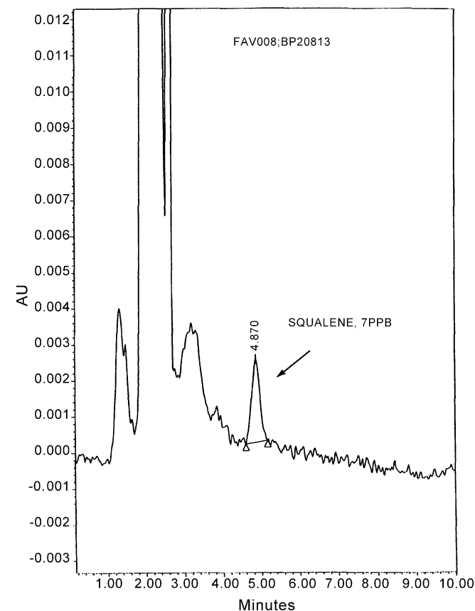
Fig. 3. Chromatogram of Lot FAV008, showing squalene at 7 \mu\text{g l}^{-1} (ppb).
