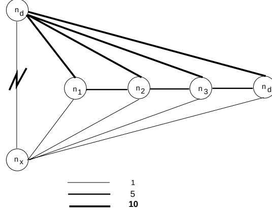
Figure 4: Complexity
