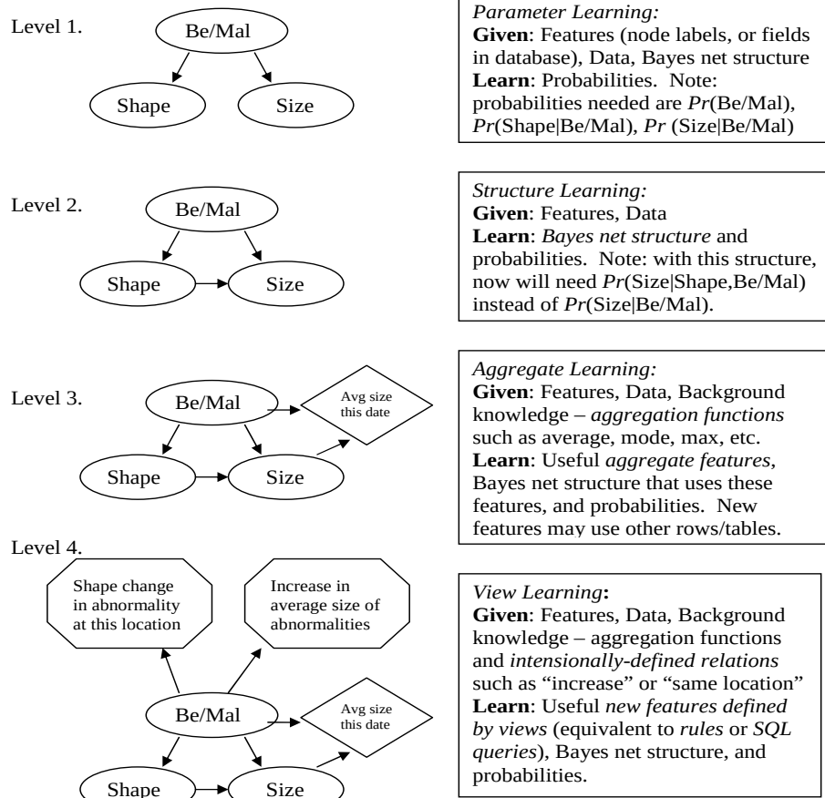
Figure 2: Hierarchy of learning types. Levels 1 and 2 are available through ordinary Bayesian network learning algorithms, Level 3 is available only through state-of-the-art SRL techniques, and Level 4 is described in this paper.
