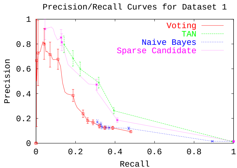
Fig. 3. P/R for Dataset 1
