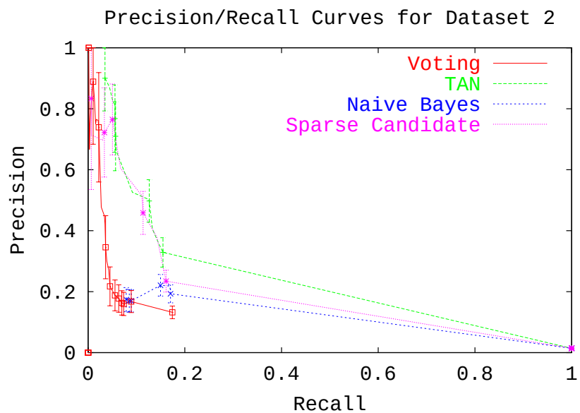
Fig. 4. P/R for Dataset 2
