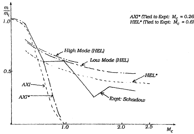
Figure 9. Mixing Ratio and Convective Mach Number in Circular Jets: Comparison Between Experiment and Theory (From Ref. [9])
