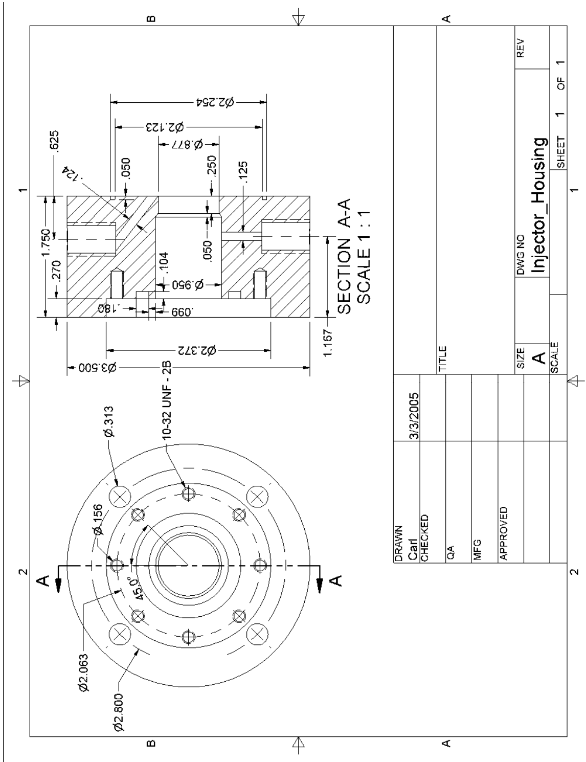
Figure 85. Injector Housing
