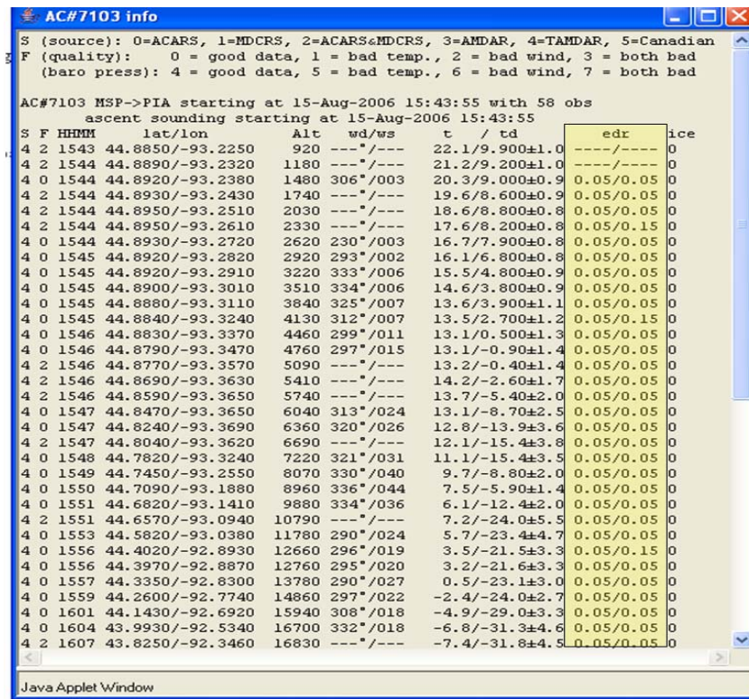
(c) Figure 78. (a) Web-based java display default load page ( http://acweb.fsl.noaa.gov/java/ ) (b) forecaster can move cursor over any EDR observation and that observation information will be displayed. (c) if forecaster right clicks on an EDR observation, a list of every EDR observation of that particular aircraft for that flight will be displayed along with it's elevation and lat/long position (EDR column is highlighted for clarity).
