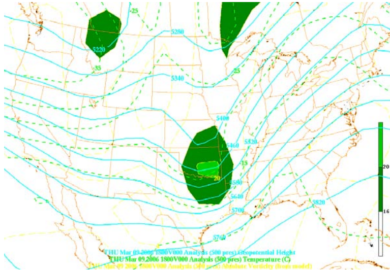
Figure 72. 500mb analysis chart for 1800 GMT, 9 March 2006 with heights (m; blue solid lines), isotherms ( ^{\circ}\text{C} ; green dashed lines), and absolute vorticity ( \text{s}^{-1} ; yellow dashed and color filled) shown.
