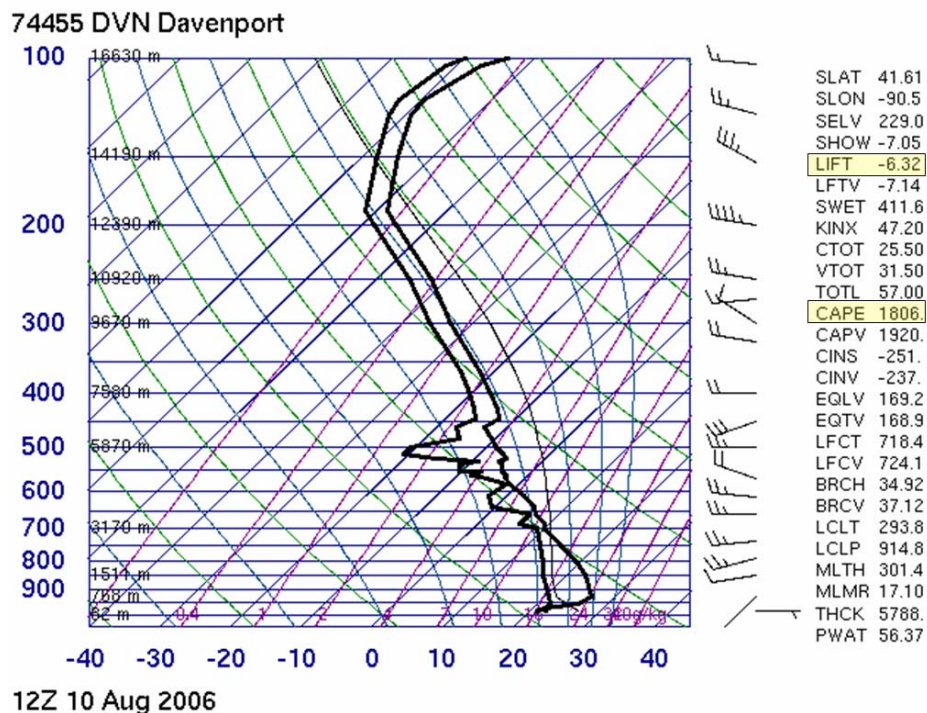
Figure 61. Atmospheric sounding for Davenport, Iowa on at 1200 GMT, 10 August 2006. The sounding has a CAPE of 1806 J/kg and a Lifted Index of -6, indicating conditions are favorable for significant convection to develop.
