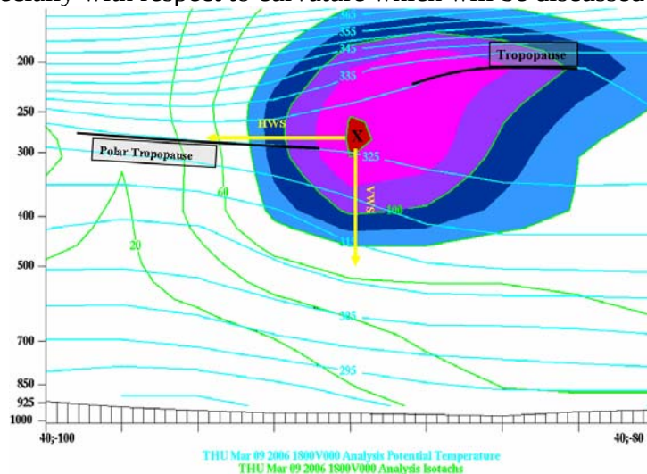
Figure 65. Cross-section from Iowa to Ohio across the jet showing isotachs (kts; solid green lines) and potential temperature ( ^{\circ}\text{K} ; solid light blue lines) for 1800 GMT, 9 March 2006. The jet is shown with the filled-in isotachs and the jet core (130 kts) is indicated by the "X". Note the strong horizontal and vertical wind shear through the jet region as shown by the yellow arrows.
