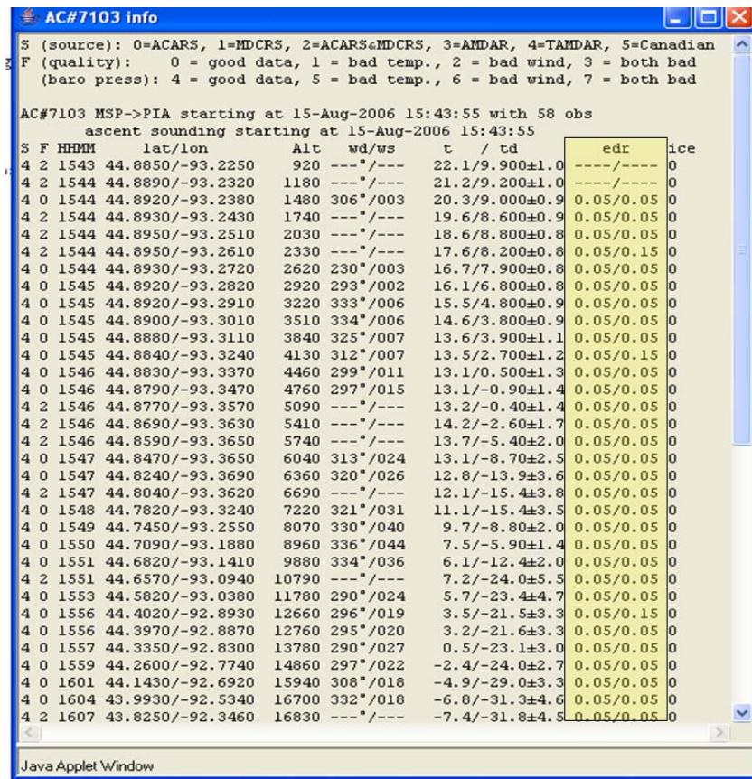
(c) Figure 44. (a) Web-based java display default load page ( http://acweb.fsl.noaa.gov/java/ ) (b) forecaster can move cursor over any EDR observation and that observation information will be displayed. (c) if forecaster right clicks on an EDR observation, a list of every EDR observation of that particular aircraft for that flight will be displayed along with it's elevation and lat/long position (EDR column is highlighted for clarity).
