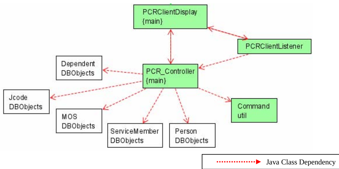
Figure 17. Presentation Layer UML Diagram
