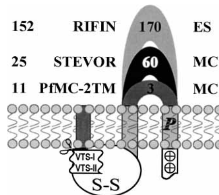
Figure 3 Schematic representation of the Plasmodium falciparum 2-transmembrane proteins encoded by subtelomeric multiplicity gene families. The number of genes and known subcellular localizations (ES, erythrocyte surface and MC, Maurer's Cleft), as well as the average number of amino acid residues in the extracellular loop are reported for the RIFIN, STEVOR, and PfMC-2TM families.
