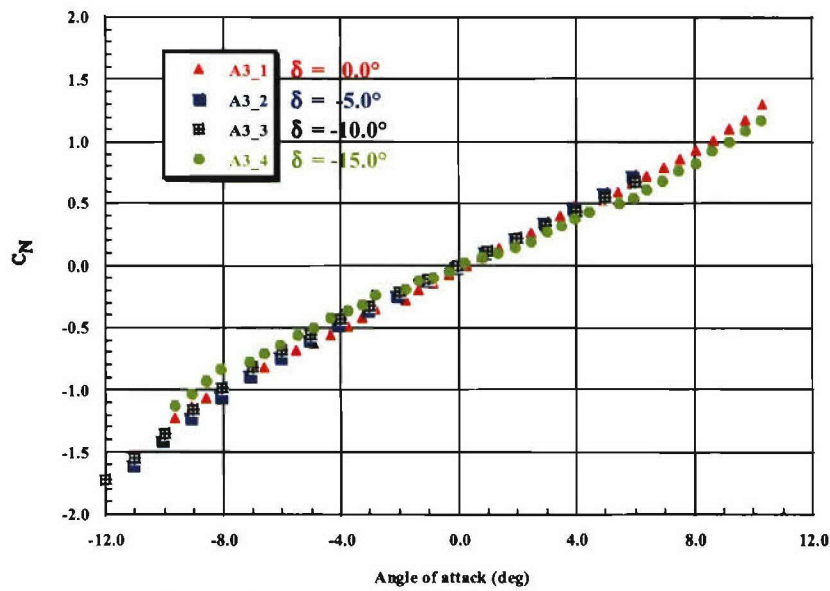
Figure 17b. Normal force coefficient vs. incidence
