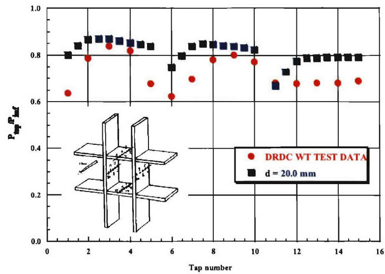
Figure 44b. Mach = 0.6, \delta = 0.0^\circ
