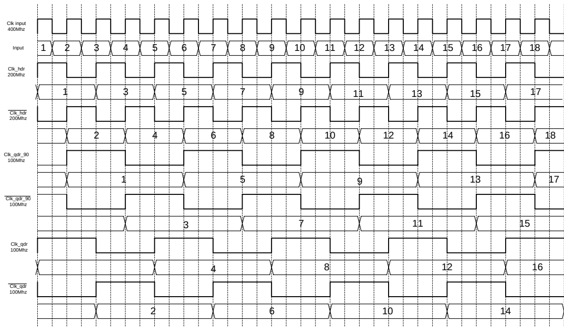
Figure 38. 400 MHz Input Register Timing diagram
