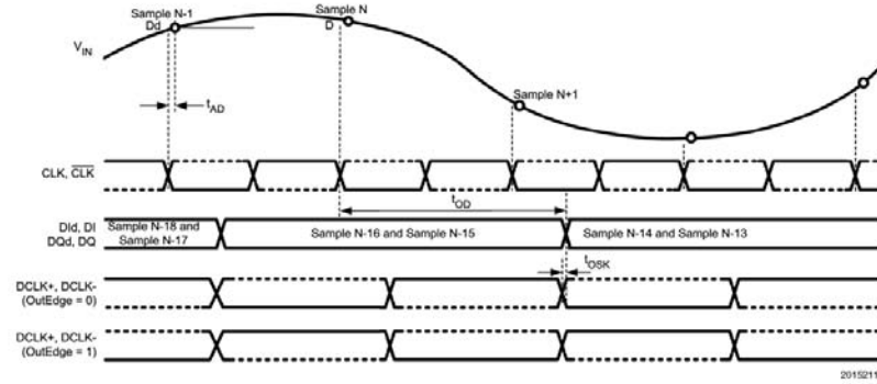
Figure 8. ADC Output Timing in SDR Mode (From [18])
