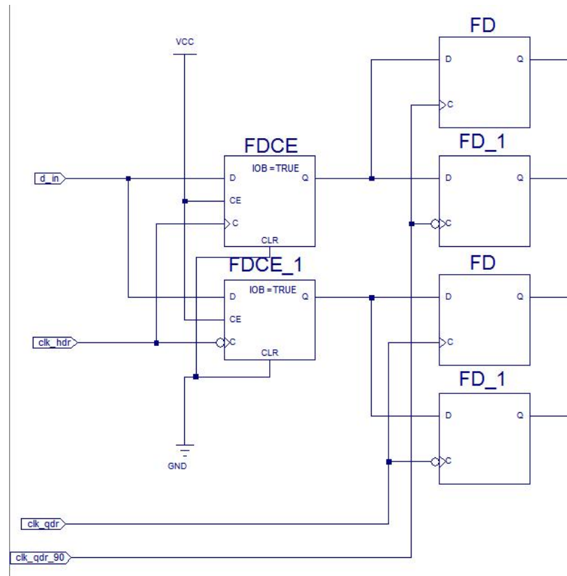
Figure 37. 400 MHz Input Register Schematic
