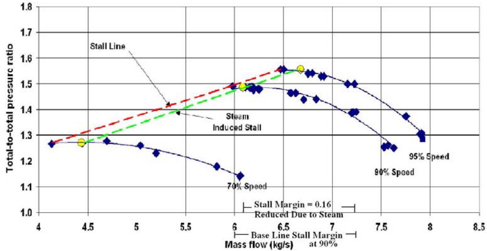
Figure 22. Compressor Pressure Ratio
