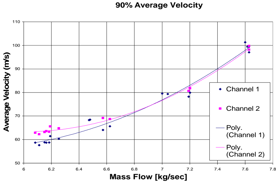
Figure 18. 90% Speed Average Velocity vs. Mass Flow Rate
