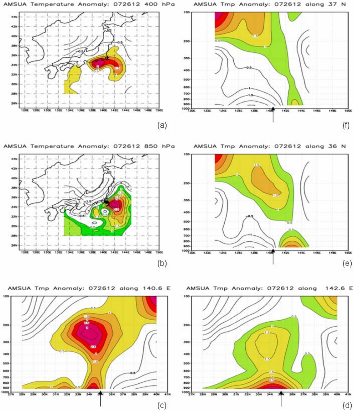
Figure 31. AMSU temperature anomaly at 1200 UTC 26 July (a) plan view, 400 hPa, (b) plan view, 850 hPa, (c) cross-section along 140.6^{\circ} E, (d) cross-section along 142.6^{\circ} E, (e) cross-section along 36^{\circ} N, (f) Cross section along 37^{\circ} N. The arrows along the abscissa indicates the position of the storm center.
