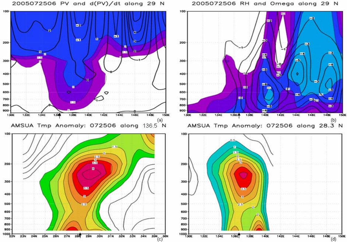
Figure 24. Zonal cross section at 0600 UTC 25 July along 29°N for (a) PV (shaded, 1 PVU = 10^{-6} K m^2 kg^{-1} s^{-1} ) and the time tendency of PV (lines, 1 PVU s^{-1} ), and (b) omega (lines, 1 \mu b s^{-1} interval) and relative humidity (percent, shaded > 80%). Temperature anomalies (K) retrieved from AMSU-A are contained in a (c) meridional cross-section along 136.5°E and (d) zonal cross-section along 28.3°N. The arrows along the abscissa indicate the position of the TC.
