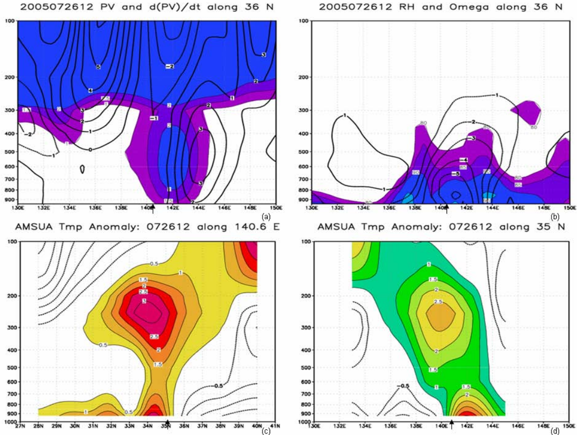
Figure 27. As in Figure 24, except for 1200 UTC 26 July, cross-sections for (a) and (b) along 36°N, for (c) along 140.6°E, and for (d) along 35°N.
