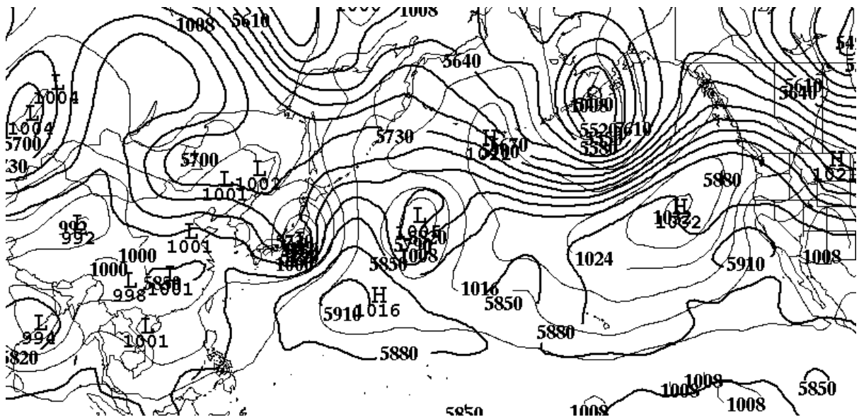
Figure 11. Same as Figure 8, except for 1200 UTC 26 July.
