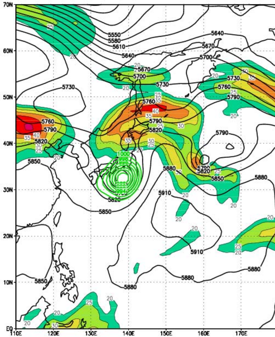
Figure 16. Same as Figure 12, except for 0000 UTC 26 July.
