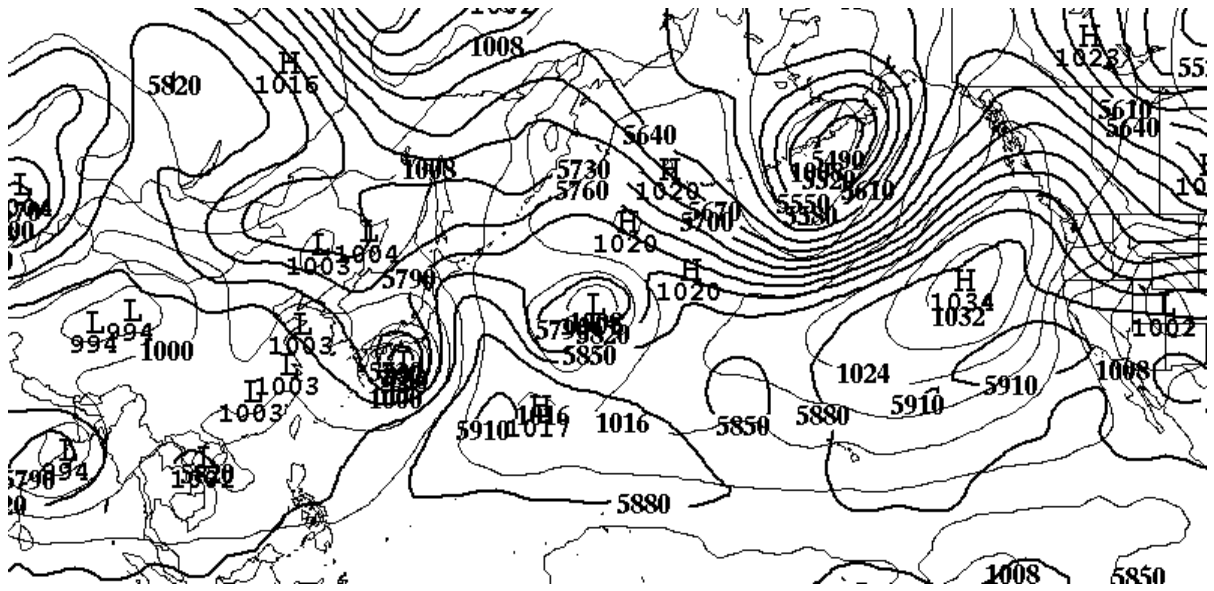
Figure 10. Same as Figure 8, except for 0000 UTC 26 July.
