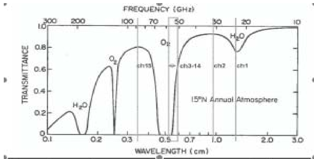
Figure 1. The AMSU-A channel frequency bands (vertical lines) as compared to the standard atmospheric water vapor and oxygen windows (curved solid lines) (after Stubblefield 2005).
