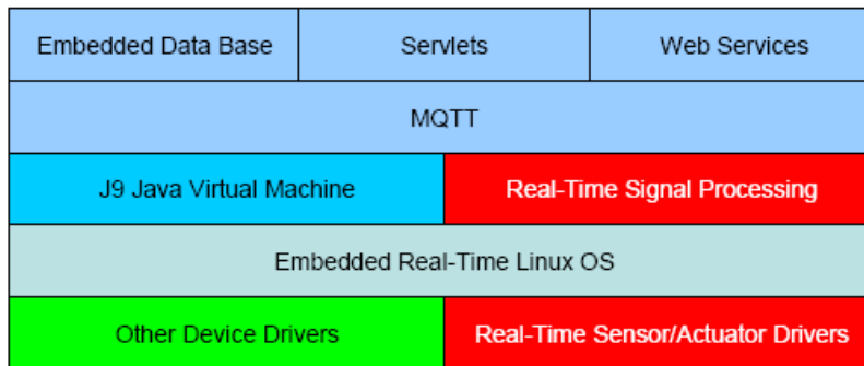
Figure 31. Software Architecture of Real-Time Sensor Controller. From: [42]
