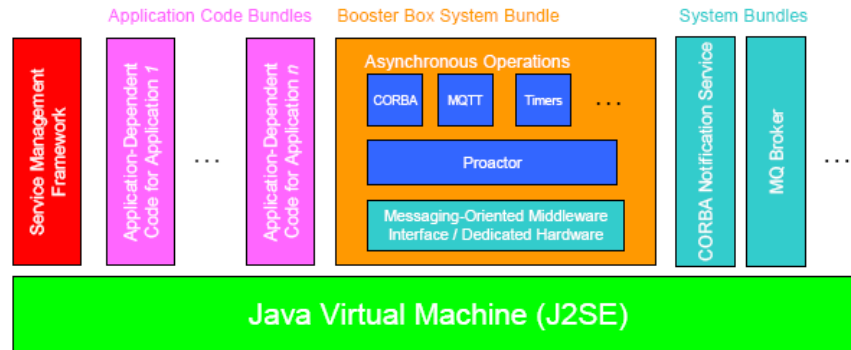
Figure 30. Software Architecture for Code Updates. From: [40]
