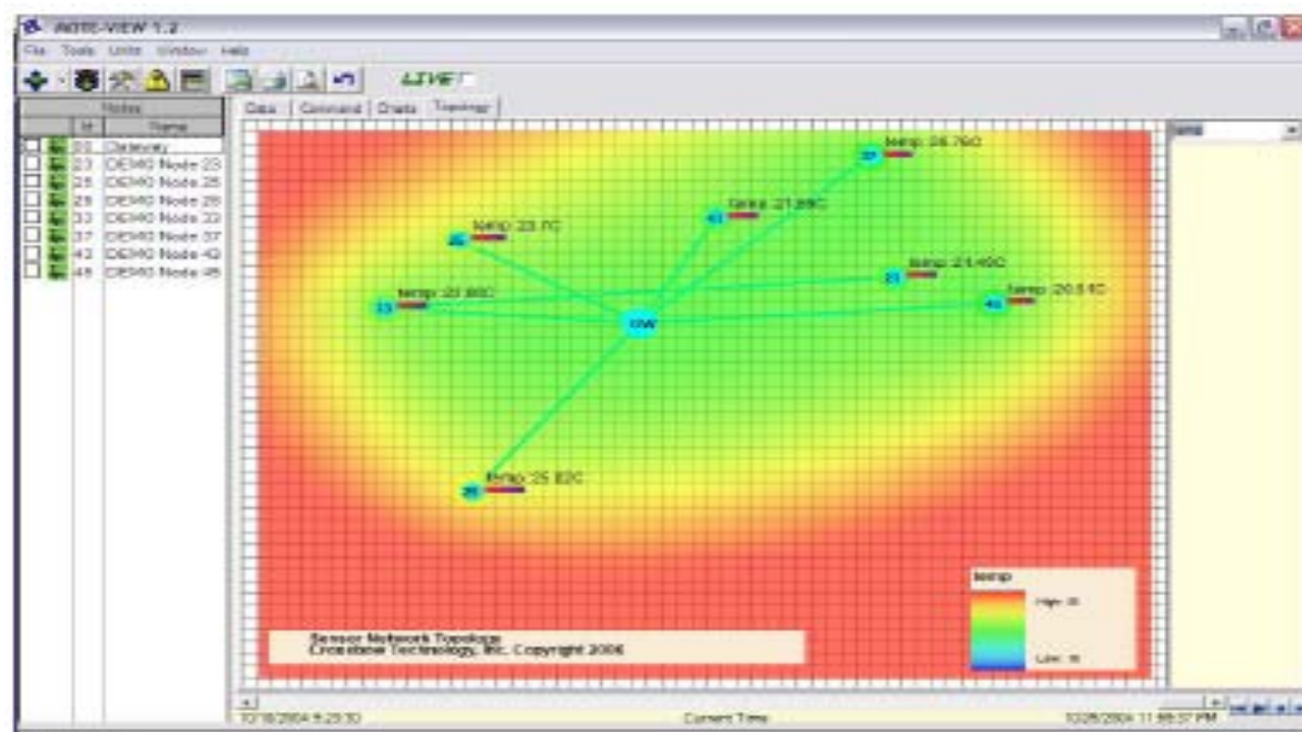
Figure 11. A topological view of the MSP410 Mote Security System depicting temperature readings in MOTE-VIEW (From: Crossbow Technology, 2006)
