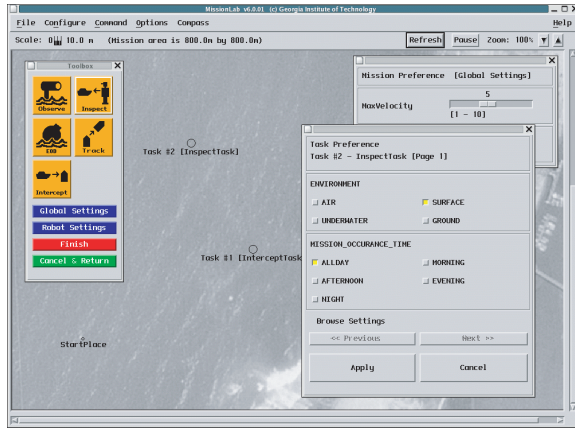
Fig. 7. The user interface for the CBR + permission-CNP design: Tasks available for placement on the left. Adjustable global parameters appear in the upper-right window. Individual task preferences are displayed and adjusted by clicking on the task location.
