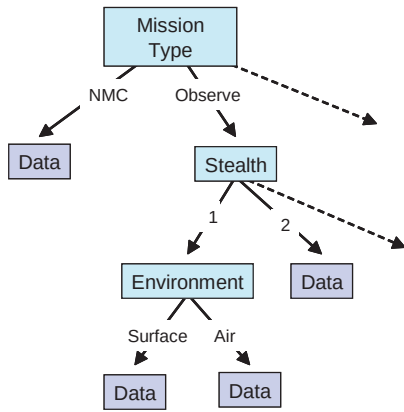
Fig. 10. Discrimination tree used to store and index cases based on specified constraints.
