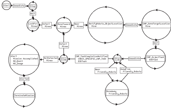
Fig. 13. FSA generated for leader robot. Its behaviors are largely for observing environmental state and injecting tasks based on that state.
