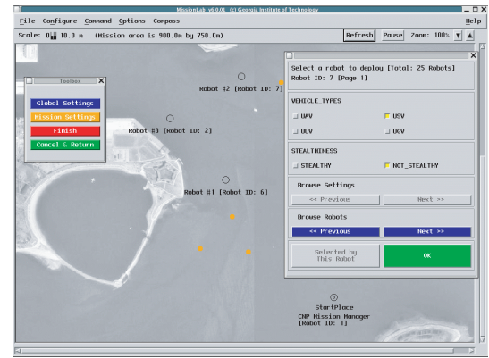
Fig. 11. The user interface for the CBR and runtime-CNP integration design: Robot selection dialog is shown on the right side of the screen.
