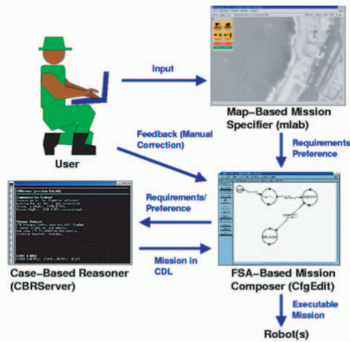
Fig. 2. Overview of mission specification using the CBR Wizard. A user specifies the desired tasks using the map-based interface of MissionLab. CBRServer retrieves a mission based on the user's input. The mission is presented for user inspection, modification, and execution.
