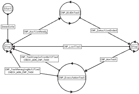
Fig. 12. FSA generated for a bidder robot. Behaviors within in it are in support of runtime task allocation.
