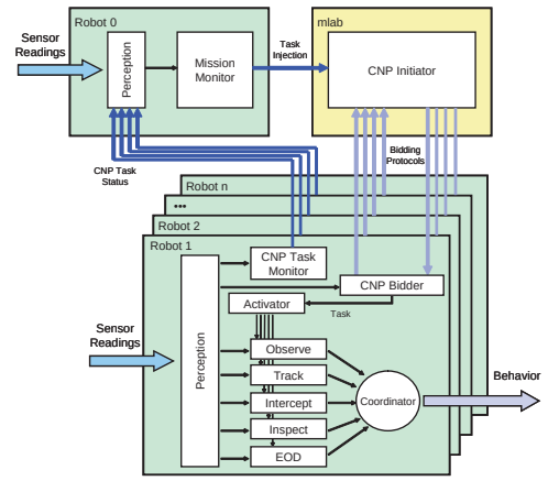
Fig. 14. Architectural framework of the execution phase for the CBR and runtime-CNP design
