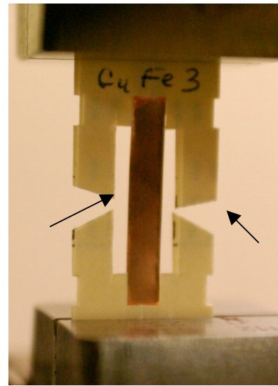
Figure 3. Photograph of the biaxially textured Cu-Fe specimen (Cu-Fe3) after the cardboard used for alignment was cut (before testing).
