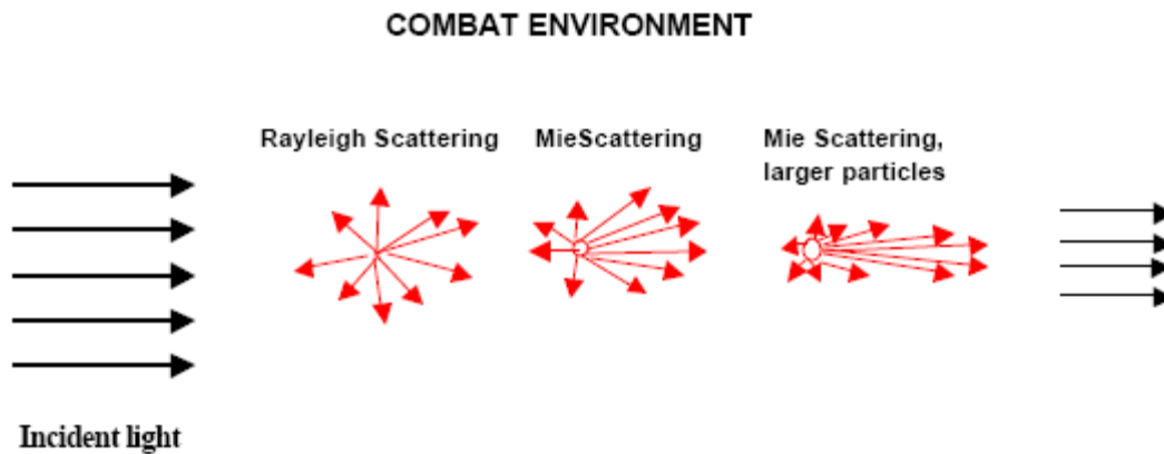
Figure 9. Rayleigh and Mie Scattering (From Ref. [11])
