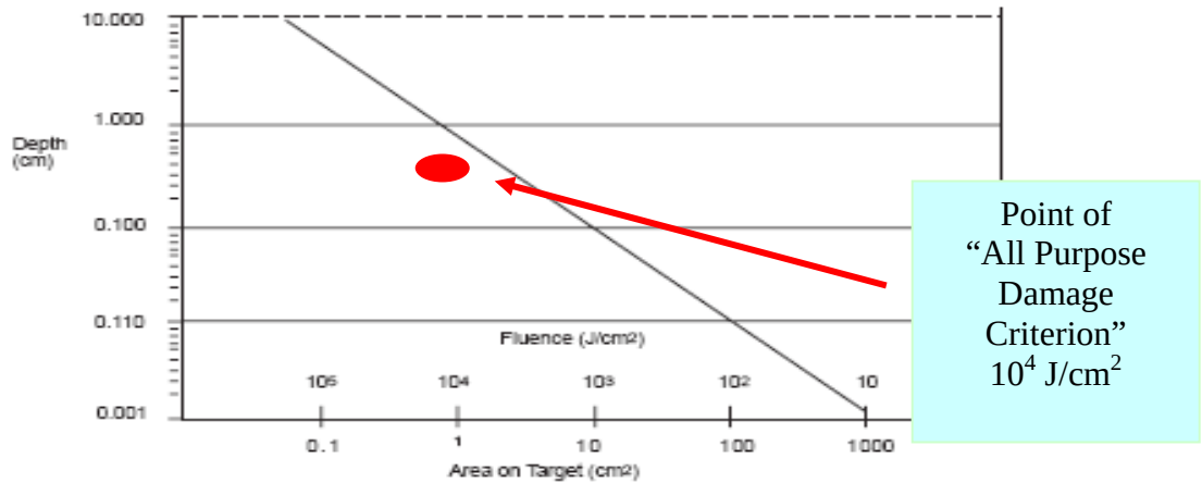
Figure 5. Depth Vaporized by 10e4 Joules versus Area Engaged and Flux (From [Ref. 7])
