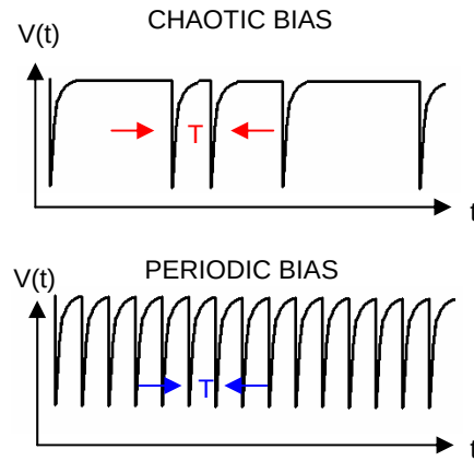
Figure 40. Output voltage is across the thyristor. The thyristor cathode is grounded.
