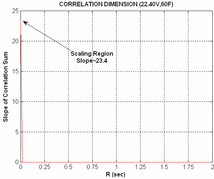
Figure 39. Correlation dimension for a periodic series.
