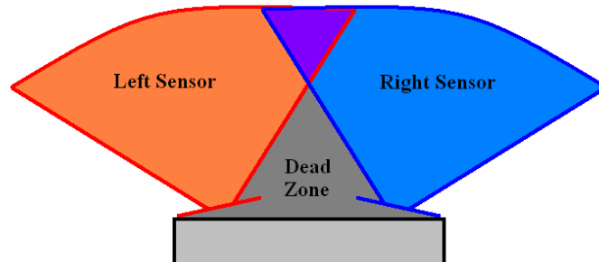
Figure 46. Sensor placement requires a shallow dead zone in front to counter the tailgating effect of one robot directly behind another.
