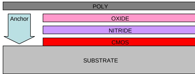
Figure 51. MEMS process.
