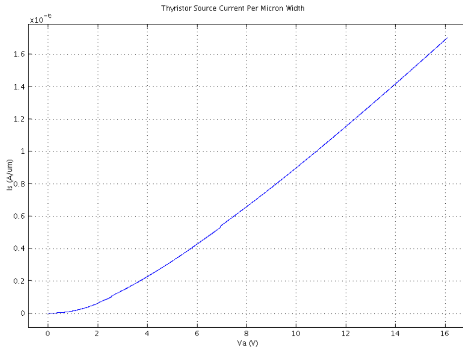
Figure 55. I-V characteristics of the thyristor. Units are A/ \mu\text{m} .
