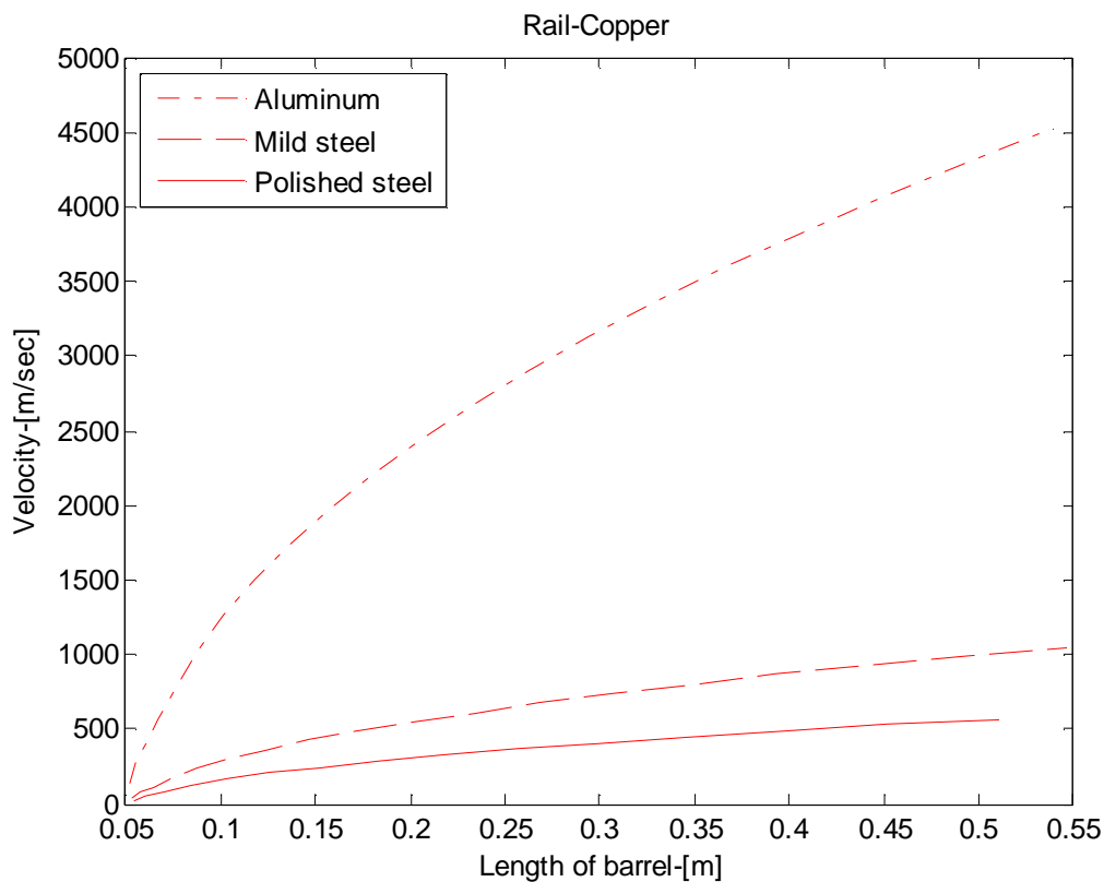
Figure 13 Velocity as a function of the displacement in the barrel for three different types of armature: a) aluminum, dotted curve b) mild steel, dashed curve c) polished steel, rigid curve
