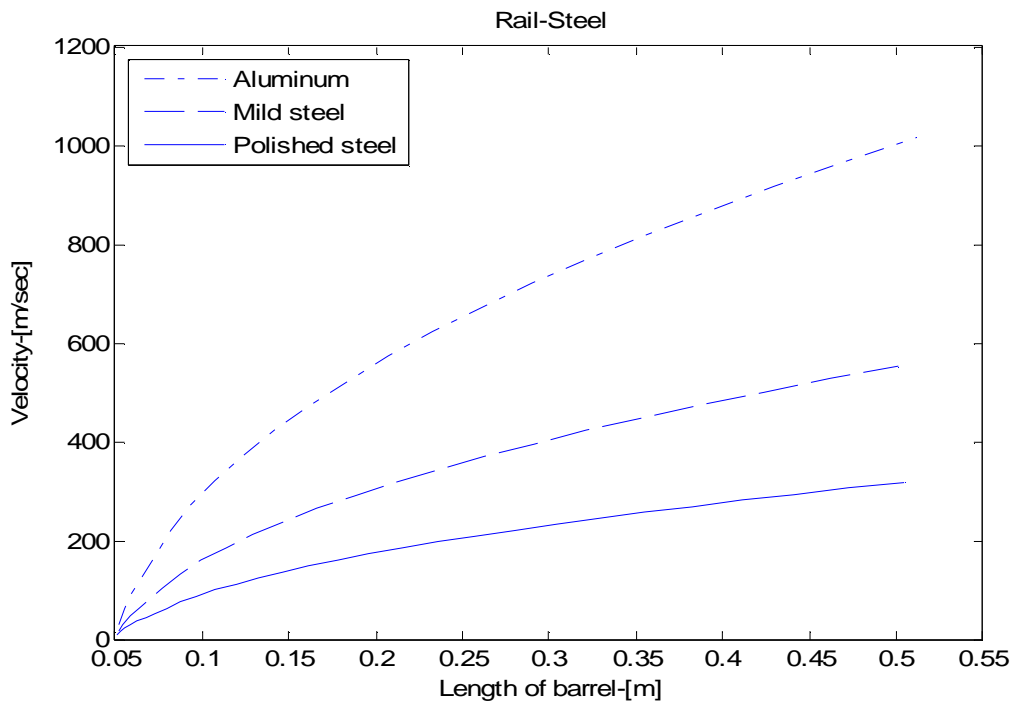
Figure 15 Velocity as a function of the displacement in the barrel for three different types of armature: a) aluminum, dotted curve b) mild steel, dashed curve c) polished steel, rigid curve
