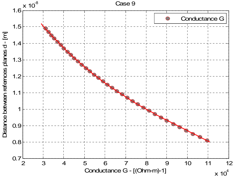
Figure 52 Case 9, Distance d between the reference planes versus conductance G
