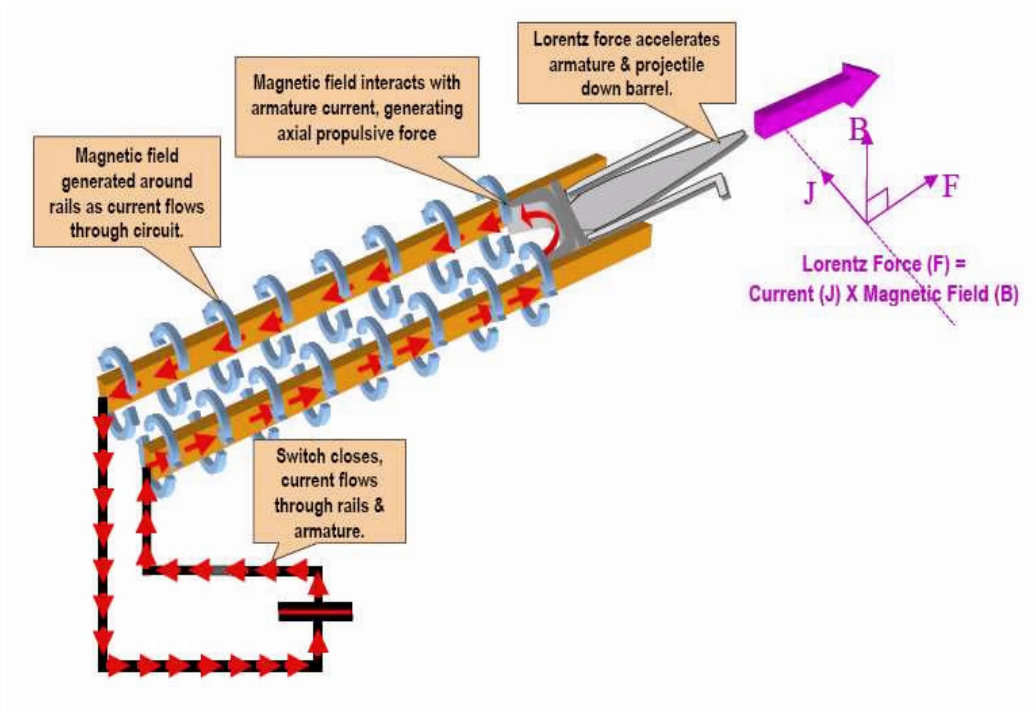
Figure 2 Schematic diagram of the principle of operation of a rail gun. [From Ref. 2]
