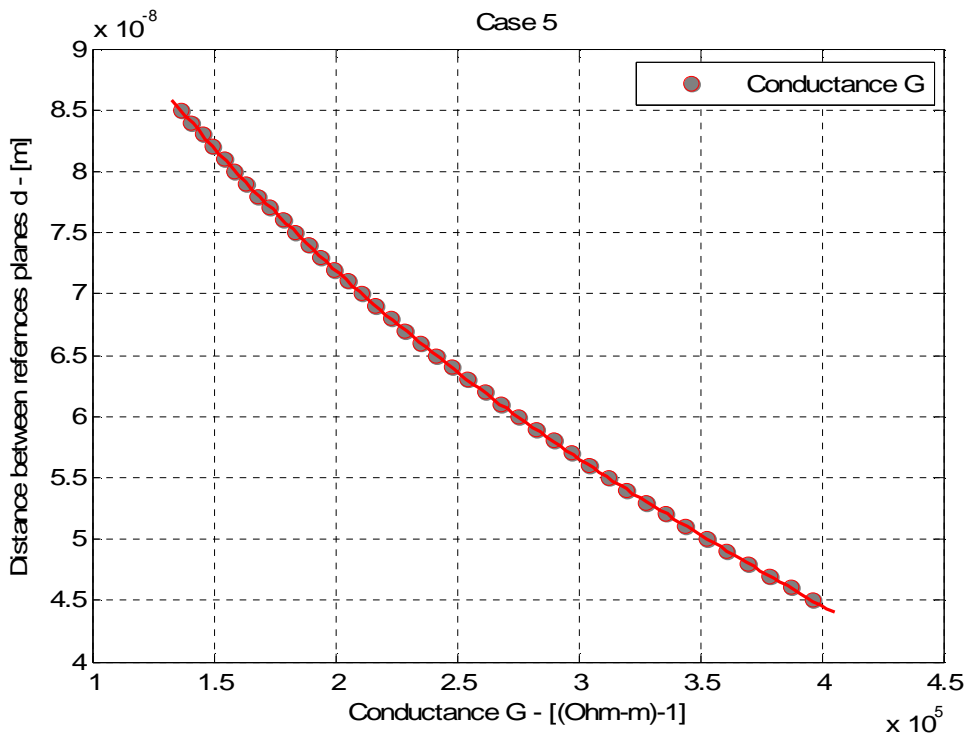
Figure 36 Case 5, Distance d between the reference planes versus conductance G
