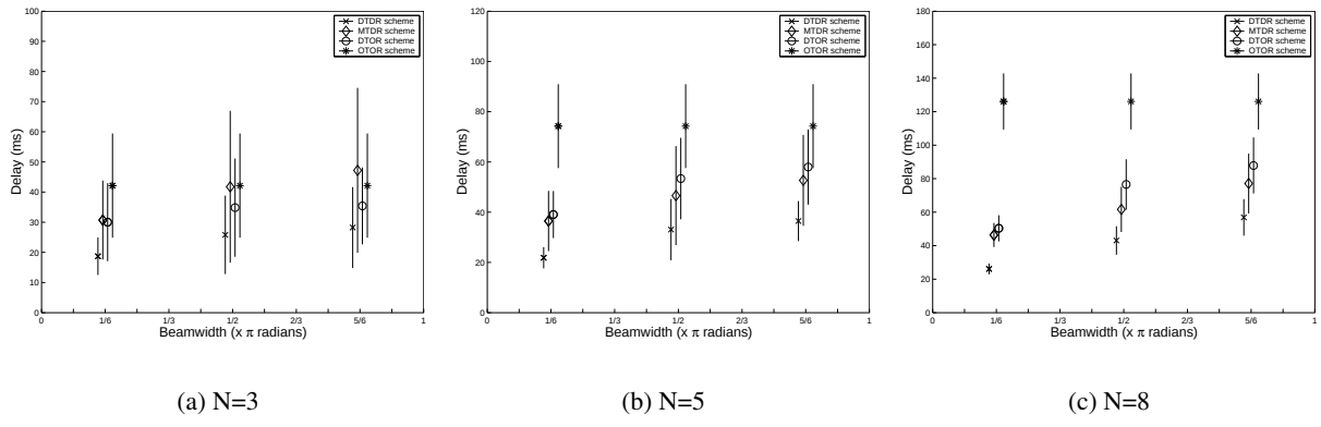
Figure 7: Delay Comparison – Equal Gain
