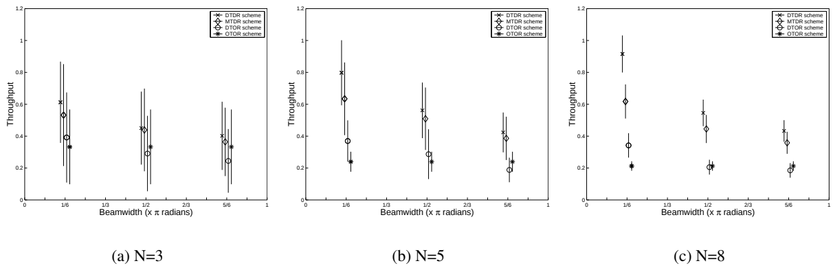
Figure 8: Throughput Comparison – Higher Gain ( \gamma = 1.5 )
