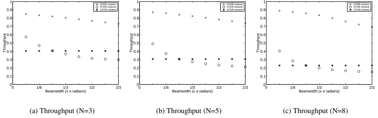
Figure 3: Throughput comparison when omni-directional and directional transmissions have equal gain ( l_{rts} = l_{cts} = l_{ack} = 5\tau, l_{data} = 100\tau, \gamma = 1 ).
