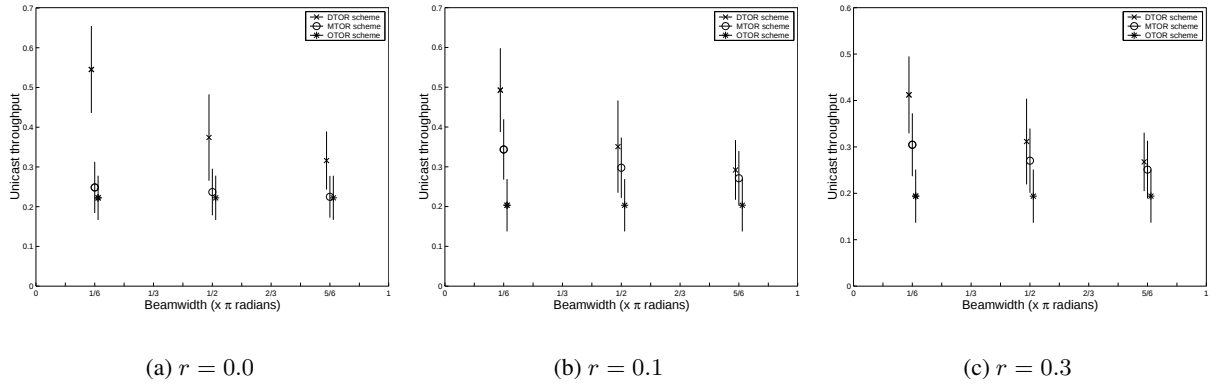
Figure 12: Unicast throughput with broadcast traffic ( N = 8 )
