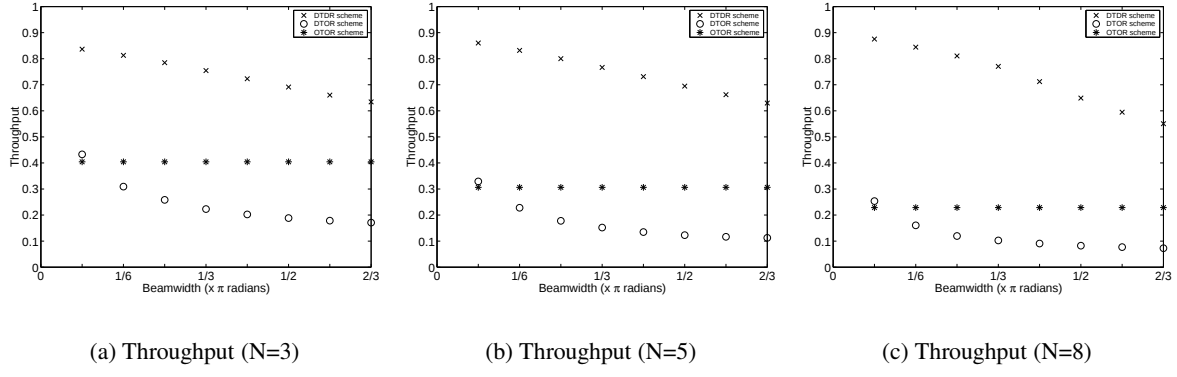
Figure 4: Throughput comparison when the gain of directional transmissions equals one and a half times the gain of omni-directional transmissions ( l_{rts} = l_{cts} = l_{ack} = 5\tau, l_{data} = 100\tau, \gamma = 1.5 ).
