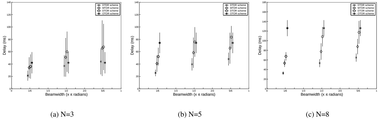
Figure 9: Delay Comparison – Higher Gain ( \gamma = 1.5 )
