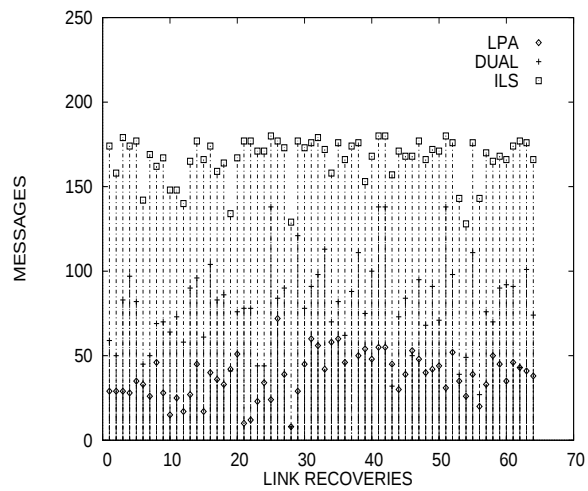
Figure 8: ARPANET Link Recovery
