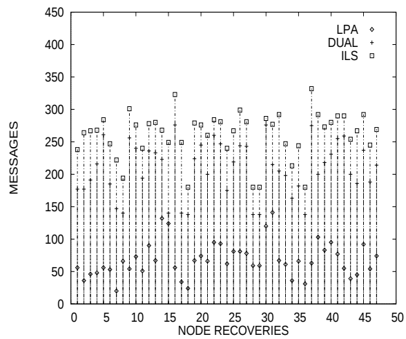
Figure 10: ARPANET Node Recovery
