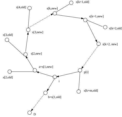
Figure 4.1: LVC loop-free condition
