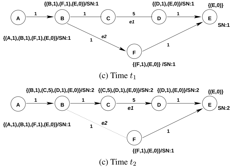
Figure 3.2: Illustration of FLR with destination-sequenced labels
