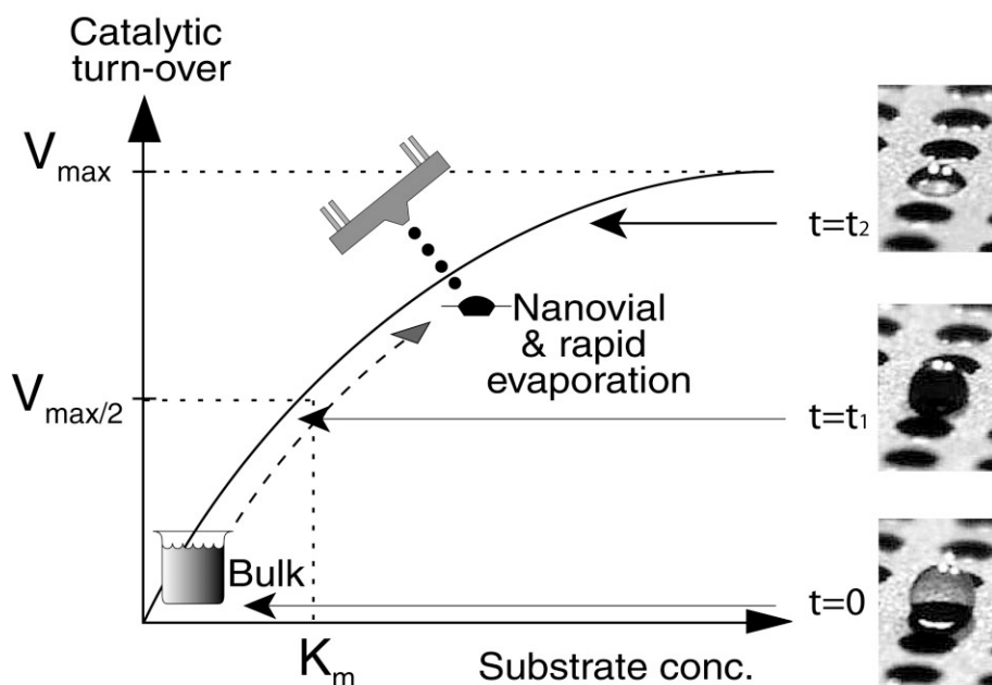
Figure 1. Schematic over the accelerated enzyme kinetics due to the substrate enrichment as the solvent evaporates from the nanovial. V_{max} is the maximal turnover rate independent of substrate concentration and K_M is equal to the substrate concentration at which the reaction rate is half of its maximal value. t = 0 , enzyme kinetics rules due to bulk solution stoichiometry; t = t_1 , substrate enrichment increases the enzymatic turn-over due to solvent evaporation; t = t_2 , maximum substrate enrichment properties have been reached, and surface area to volume ratio becomes dominant. Hence, surface-bound catalysis further accelerates the digestion process.
