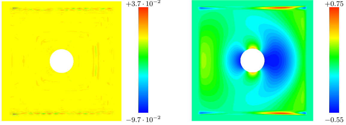
Figure 11: Electromagnetic scattering of a plane wave on a cylinder. Left: Real part of the second component of the error estimate; k = 2\pi . Right: Real part of the second component of the numerical solution; k = 1 .
