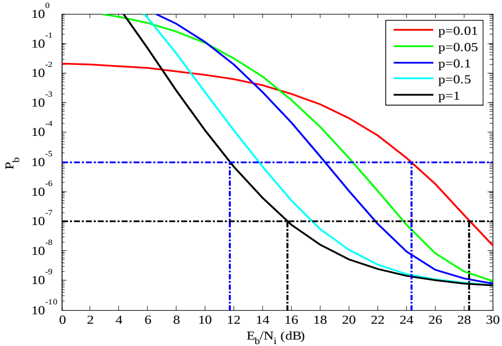
Figure 29. Performance of r=2/3 , K=2 convolutional code with 8-BOK, HDD and PNI with E_b/N_0 = 10.394 dB
