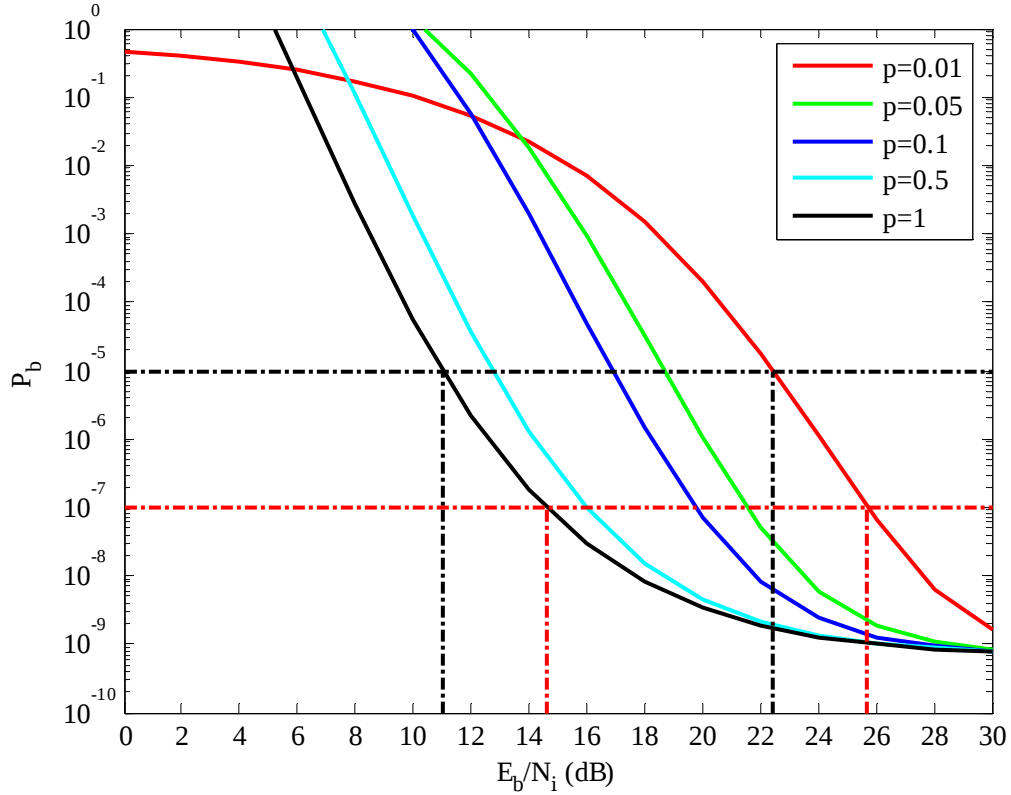
Figure 39. Performance of r=3/4 , K=6 convolutional code with 16-BOK, HDD and PNI with E_b/N_o = 7.82 dB
