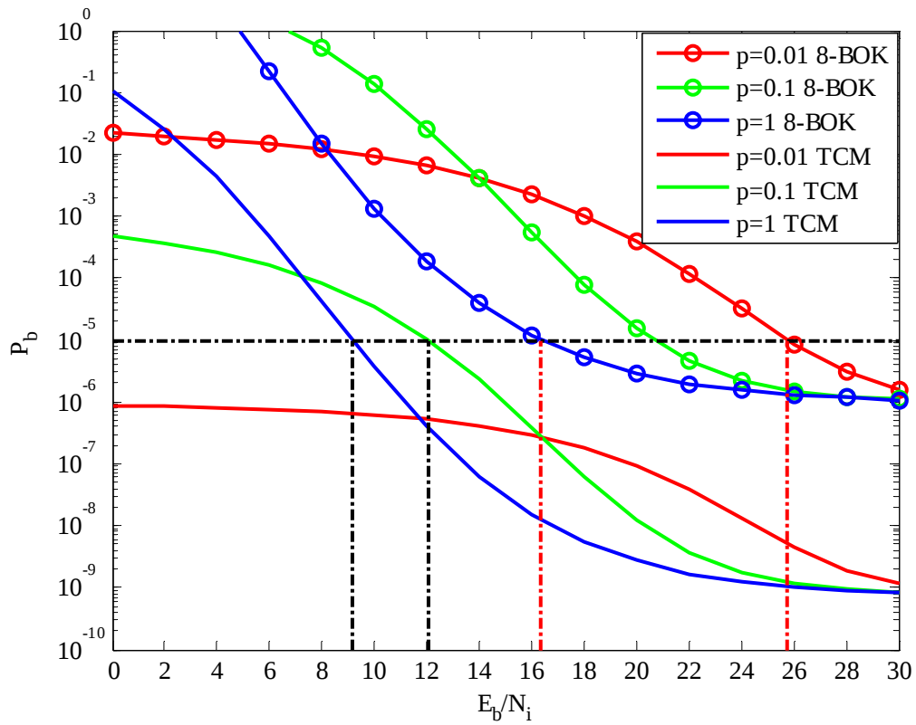
Figure 33. Comparison of r=1/2, v=3 convolutional code with QPSK TCM PNI and r=2/3, K=2 convolutional code with 8-BOK HDD and PNI with E_b/N_o = 8.691 dB
