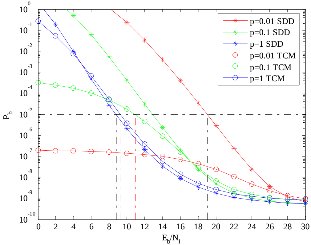
Figure 27. Comparison of r=1/2, v=4 convolutional code with QPSK TCM PNI and r=1/2, v=4 convolutional code with QPSK LC and PNI with E_b/N_o = 8.123 dB
