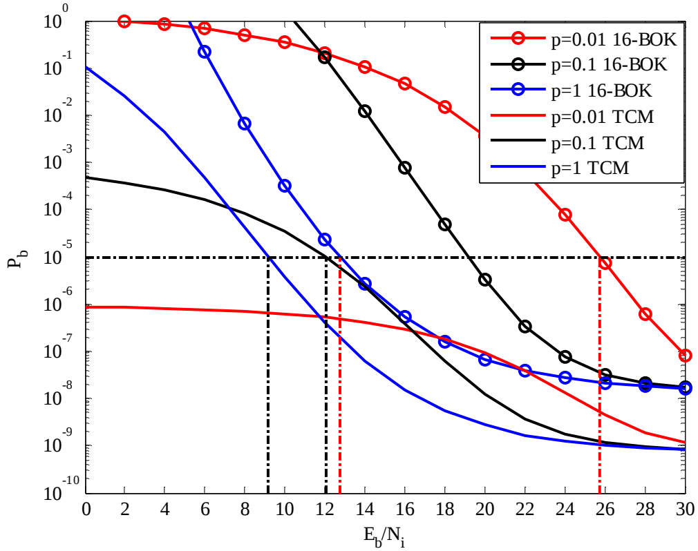
Figure 40. Comparison of r=1/2, v=3 convolutional code with QPSK TCM PNI and r=3/4, K=2 convolutional code with 16-BOK HDD and PNI with E_b/N_o = 8.691\text{dB}
