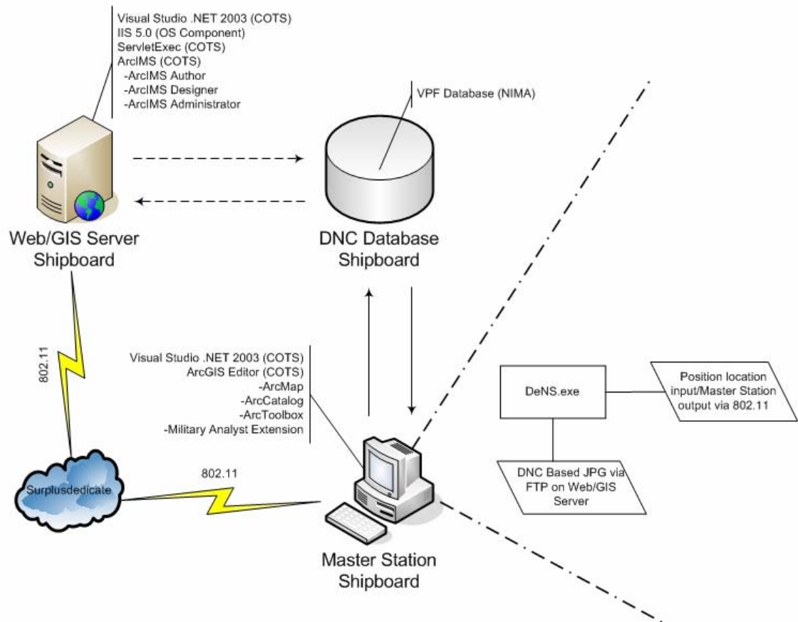
Figure 7. DeNS Architecture
