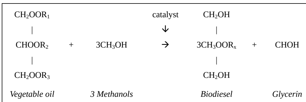
Figure 3. Biodiesel production.
