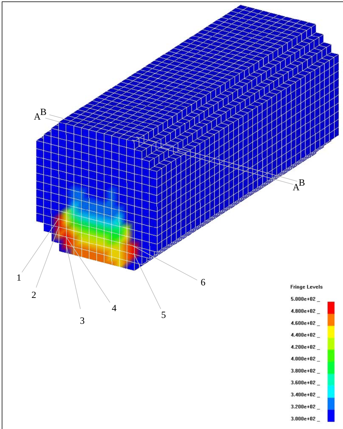
Figure 17. The initial temperature field in the M30A1 grain, and the six nodes at which temperature histories are provided in figure 18. (The fringe levels are in Kelvin.)
