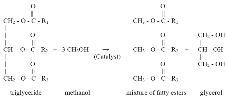
Figure 8. Transesterification reaction.
