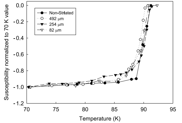
Fig. 5. dc Susceptibility curves for all samples.
