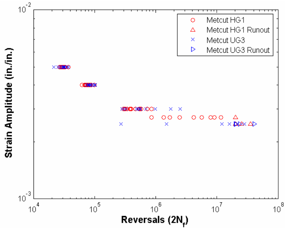
Figure 16: Strain-Life Scatter of Metcut HG1 and UG3 Coupons, Initial Overstrained
