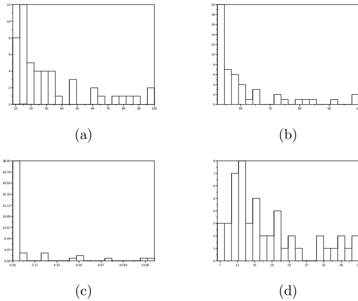
Figure 6.4: Distribution of centralities in a scale-free network: (a)Degree, (b)Closeness, (c)Betweenness, and (d)Eigenvector
