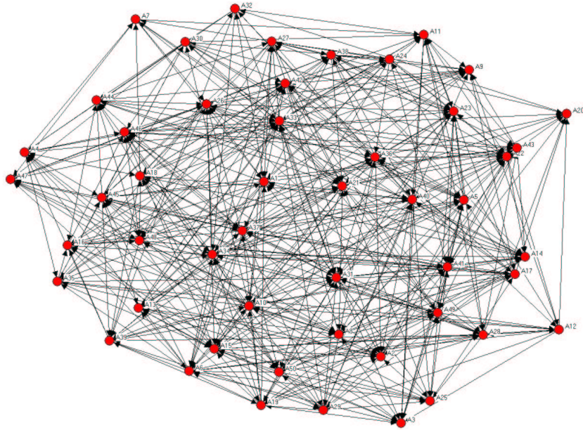
Figure 6.1: A Uniform Random Network
