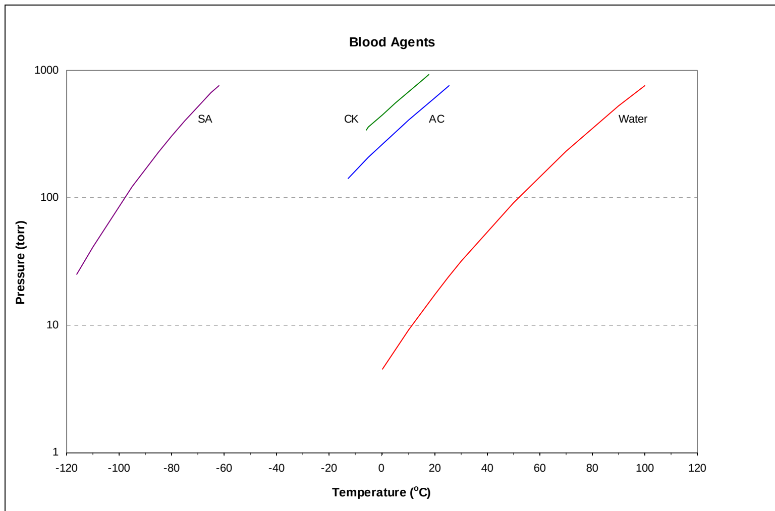
Figure G-3. Vapor Pressure of Blood Agents 1
