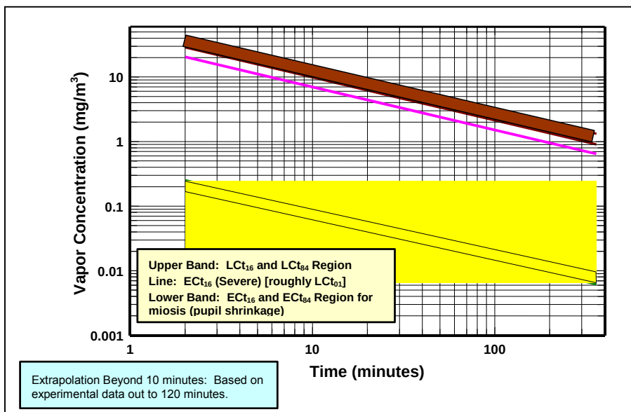
Figure H-2. GA Vapor: Concentration versus Exposure Duration
