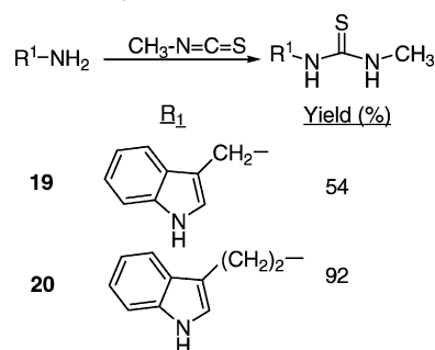
Scheme 4. Brassinin Synthesis
