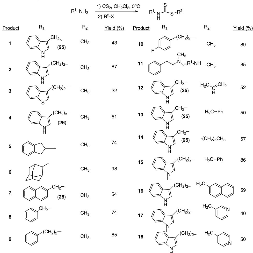
Scheme 3. Thiourea Synthesis
