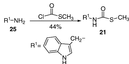
Scheme 4. Brassinin Synthesis
