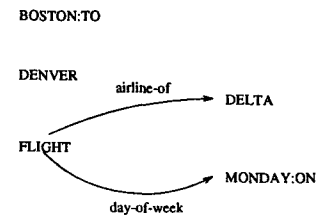
Figure 3: Fragment Graphs
