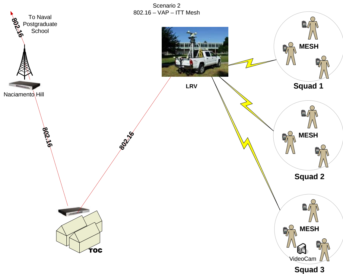
Figure 27. Scenario Two 802.16 Backhaul to Mesh Access Layer Integration
