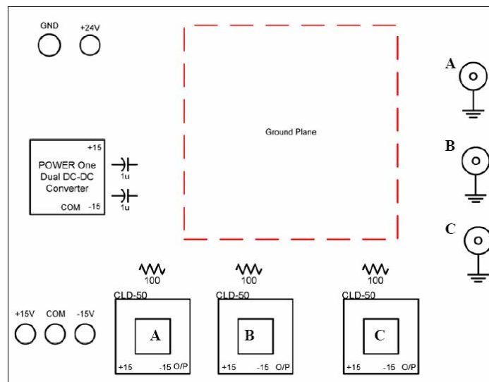
Figure 43 Hall Effect Sensor Layout
