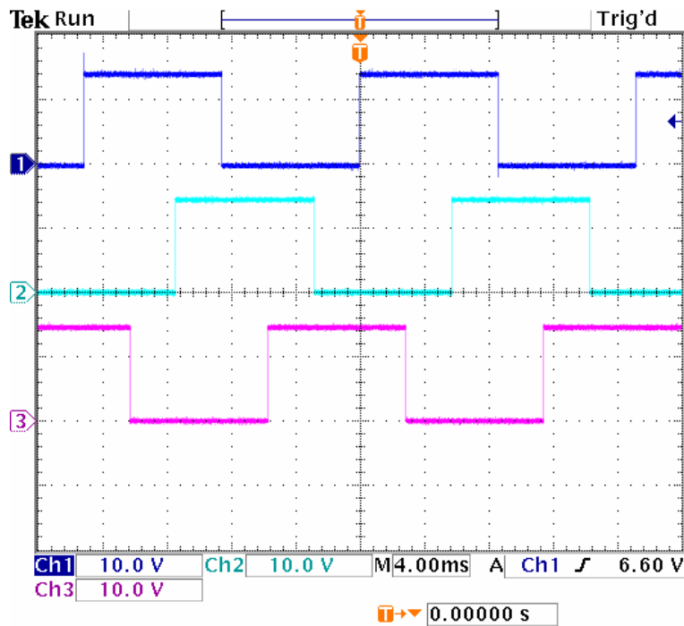
Figure 46 Gating Signals
