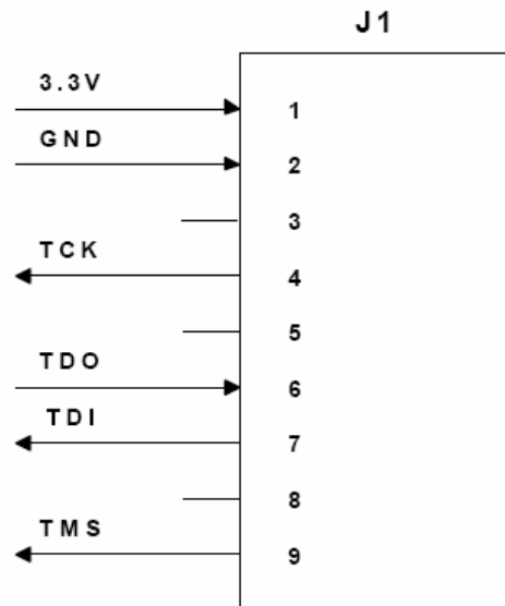
Figure 57 JTAG Connection Diagram [From Ref 16]
