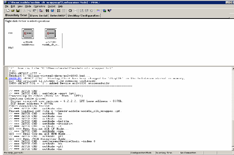
Figure 42 XILINX® iMPACT™
