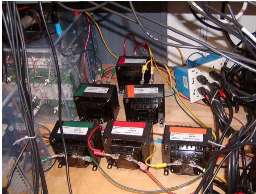
Figure 30 Conditioning Reactors
