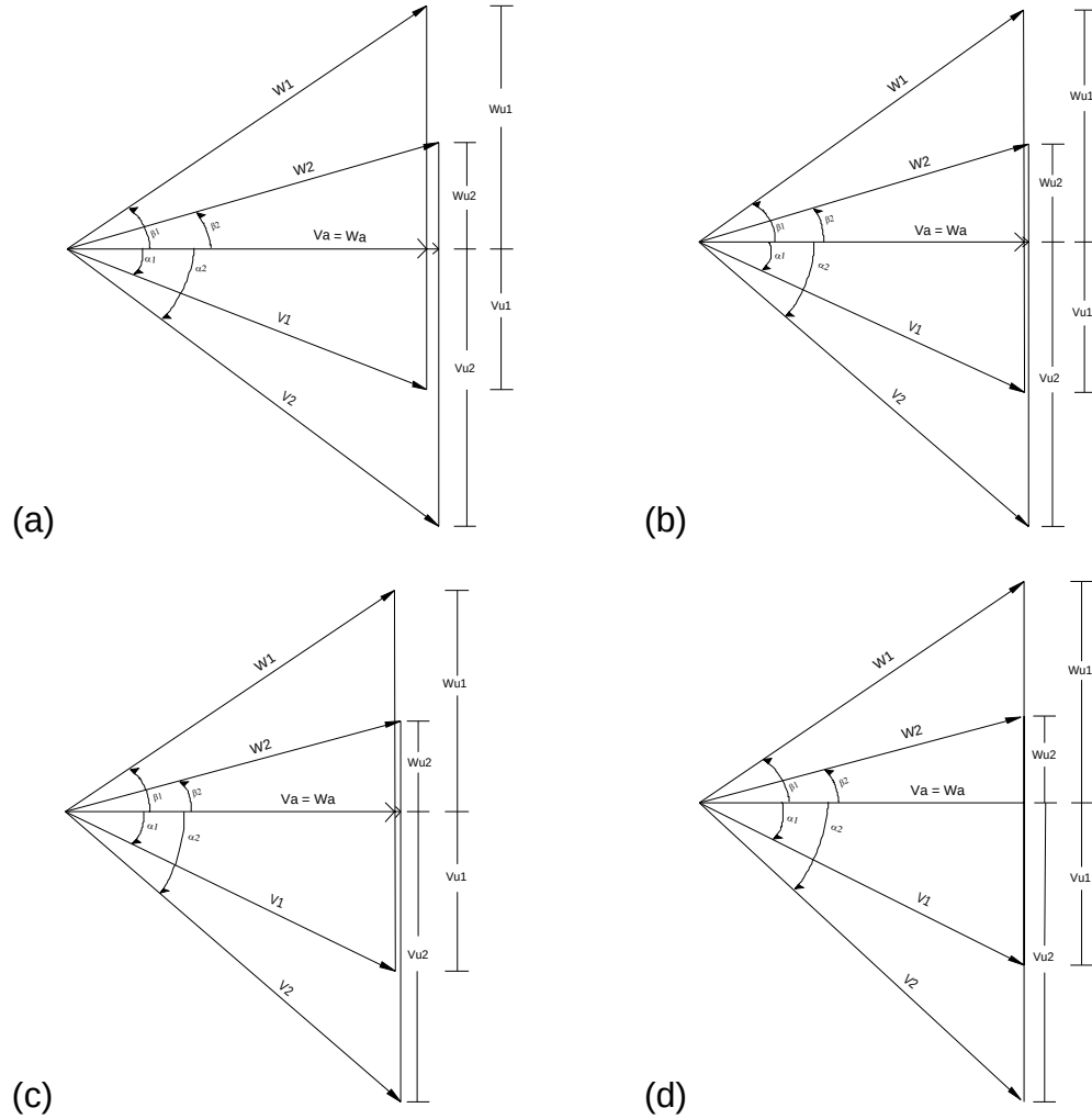
Figure E5. Point location #5 – (a) Open throttle (b) Throttle 5+4 (c) NOP (d) Near stall
