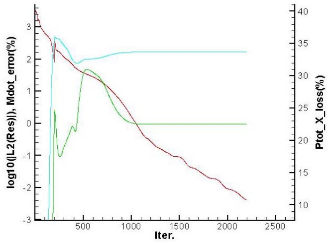
Figure 34, Convergence History for Iteration 28 Analysis
