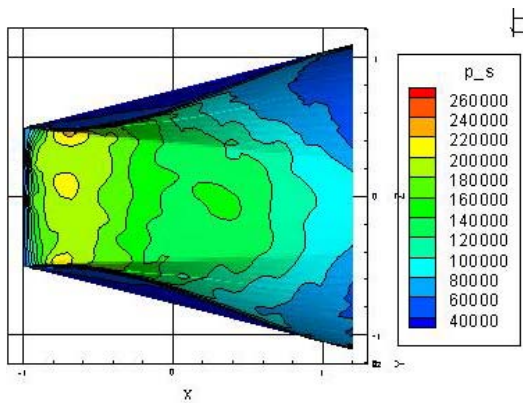
Figure 16, Uniform Inflow Side-Wall Pressure Contour Plot - Baseline
