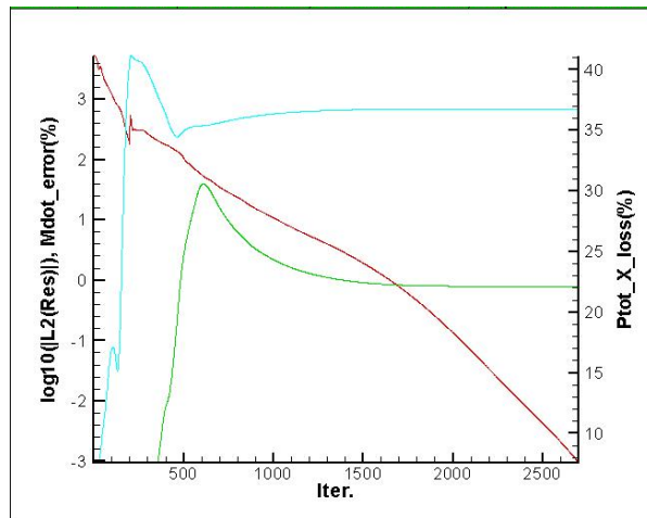
Figure 30, Convergence and FOM History for Iteration 29 of the Optimization Using OD Distortion
