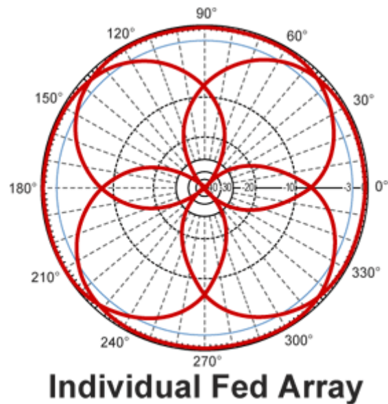
Figure 26. RF Propagation from the Sectorfed Omni Array
