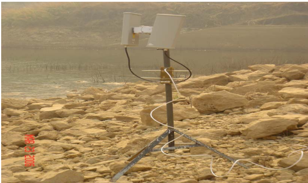
Figure 52. 180 degree array used at the Mae Ngat Dam during testing
