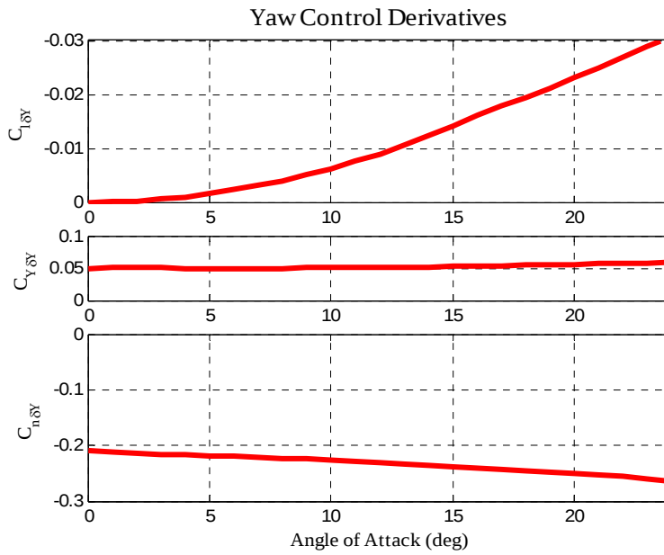
Figure 18. Yaw control Derivatives
