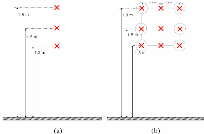
Fig 3. The measurement position at open site (a) and non-open site (b) (circles are applied when 6 points are used)
