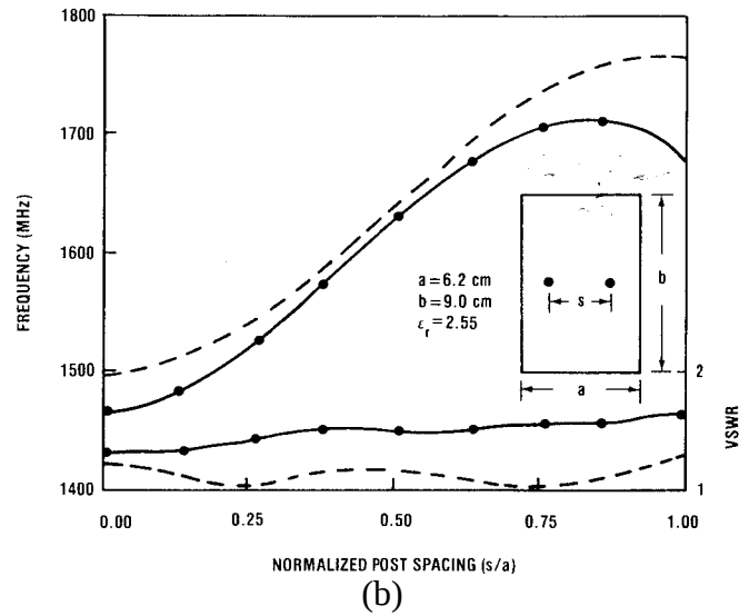
Figure 8. Post-tuned microstrip patch antenna inspired by work in [10], [11] and [14]. (a) Antenna with pair of posts separated by distance s . (b) Frequency tuning and VSWR of post-tuned antenna, from [15].
