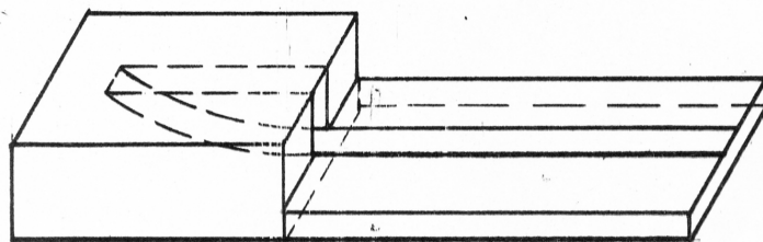
WAVEGUIDE TO MICROSTRIP TRANSDUCER FIG. 2
