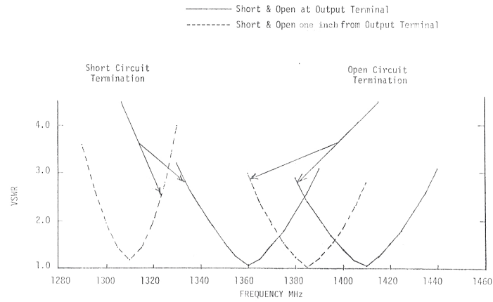
Figure 3. Kerr's results for frequency tuning by open-circuit and short-circuit loads at two locations. From [11].
