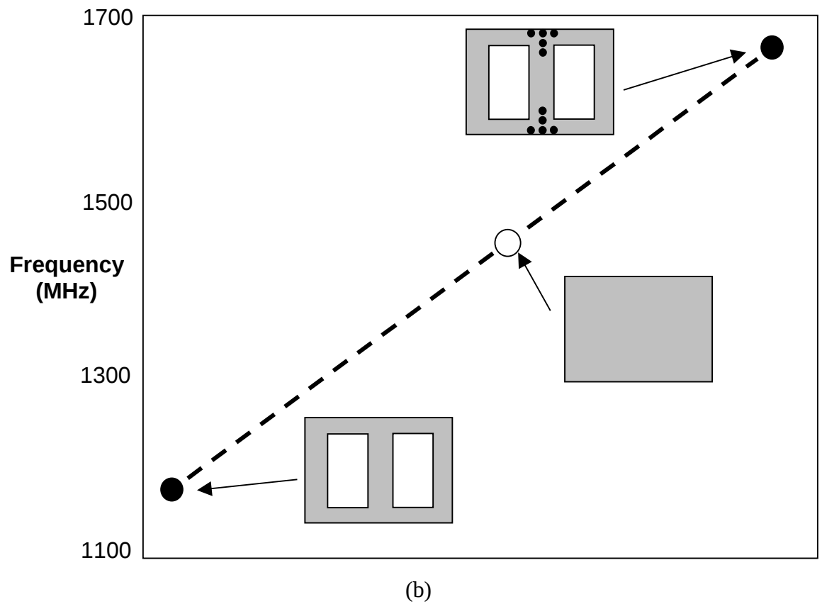
Figure 9. (a) Patch antenna with metalization removed to lower basic operating frequency and posts added to then raise it. (b) Typical tuning range of patch antenna. Standard patch antenna of same size operates at 1465 MHz. After [16].
