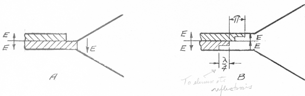
SANDWICH-LINE TO HORN TRANSITIONS FIG. 7
