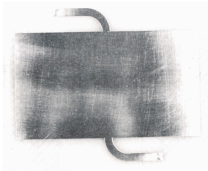
Figure 2. Terminated microstrip antenna demonstrating frequency tuning by reactive loading of the patch. From [11].
