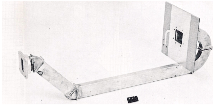
Figure 1. Kerr's L-band patch antenna with hole for X-band feed horn. From [10].
