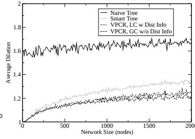
Figure 4: Dilation as network size is increased.
