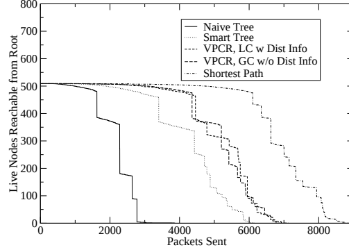
Figure 7: Network Lifetime
