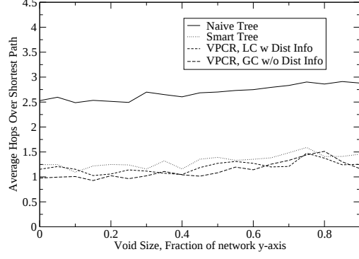
Figure 12: Performance in the presence of a void that extends vertically from one side of the network to the other.
