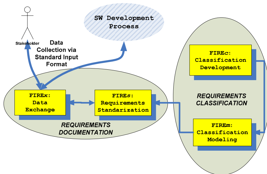
Figure 5. Activities required for the integration of evolving requirements.
