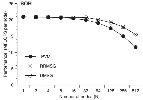
Figure 9.8: Per-node performance of a 4096 \times 4096 element SOR for different machine sizes.
