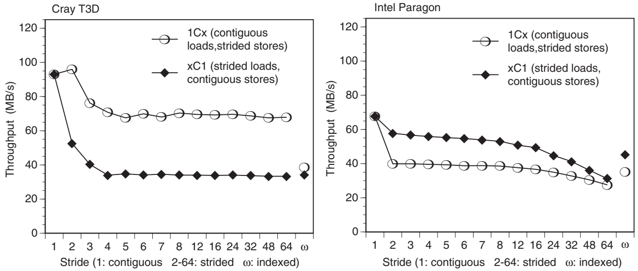
Figure 9.20: Throughput for strided local memory-to-memory transfers (MB/s).
