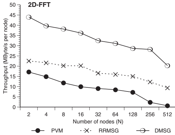
Figure 9.11: Per-node communication performance of a 4096 \times 4096 point 2D-FFT for different T3D machine sizes.
