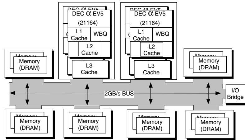
Figure 2.6: Overview of the DEC 8400 system architecture. The “communication” system comprises a high speed bus with several slots to incorporate processor, memory and I/O modules.
