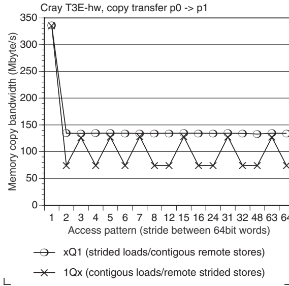
Figure 8.20: Measured performance of large remote copy transfers (i.e. between processors) on the Cray T3E for different strides. Note the different scale.
