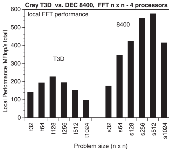
Figure 9.28: Local computation performance of the 2D-FFT benchmark on 4 processors of a Cray T3D (left) and a DEC 8400 (right). Benchmark written in Fx Fortran.
