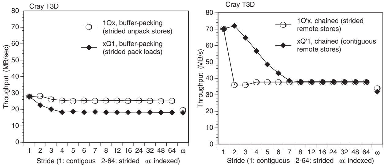
Figure 9.25: Throughput for communication operation with different strided access patterns including contiguous, strided and indexed for either loads or stores. The buffer-packing implementations (left) result in a lower throughput than the chained implementations (right).
