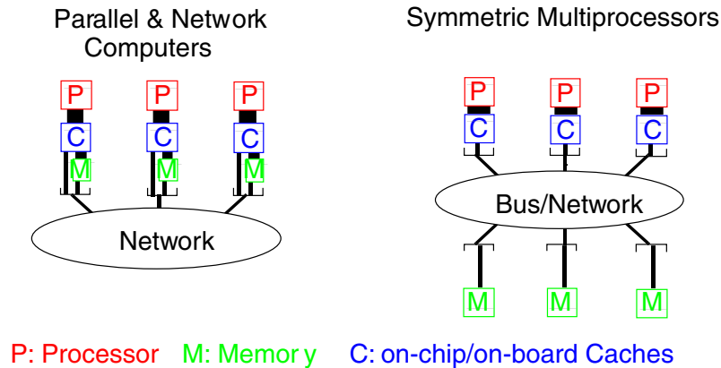
Figure 2.1: The overall layout of the memory system and the amount of hardware support for coherency are the factors that distinguish between distributed and shared memory architectures. The memory system performance can vary in both types of machines.
