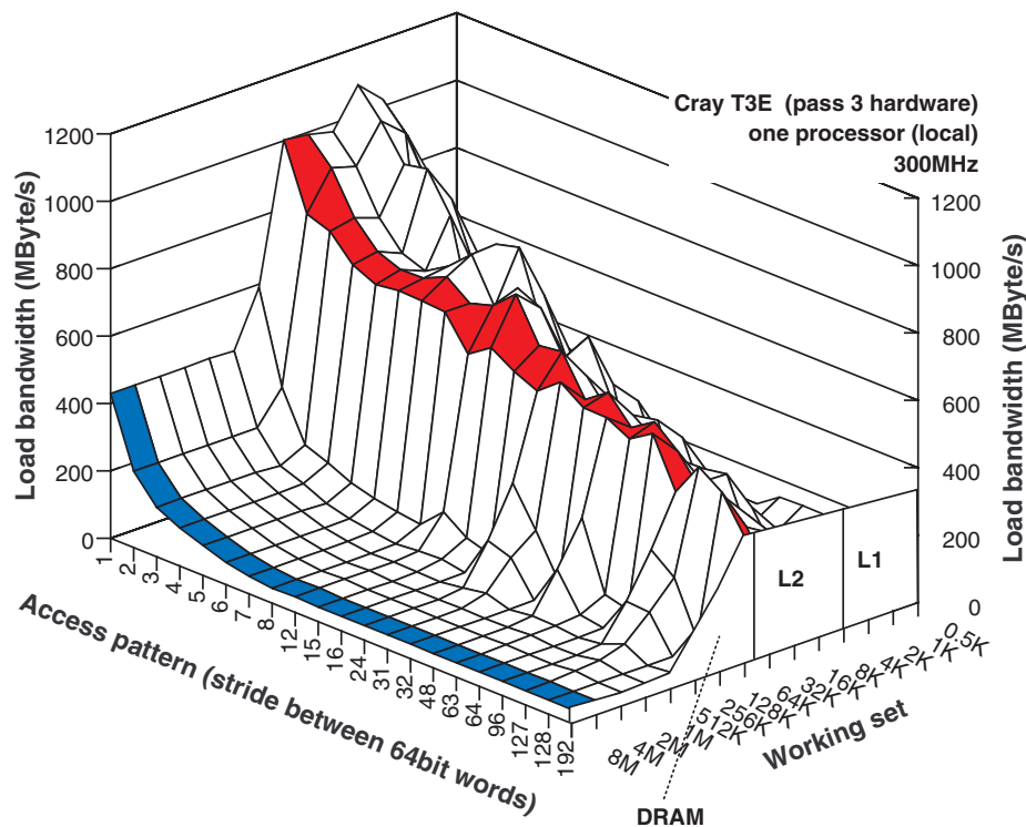
Figure 8.9: Cray T3E: Load bandwidth for different access patterns (strides) and different working sets. One processor runs the memory benchmark, and the other three processors idle.
