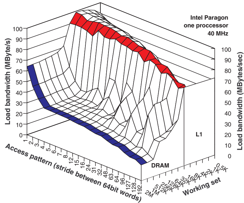
Figure 8.12: Intel Paragon: Load bandwidth for different access patterns (strides) and different working sets. Benchmark executes on a single node.
