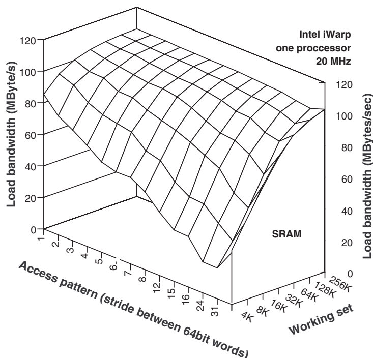
Figure 8.15: Intel iWarp: Load bandwidth for different access patterns (strides) and different working sets. Benchmark executes on a single node. Important note: The axis of the working set had to be reversed to allow proper visualization.
