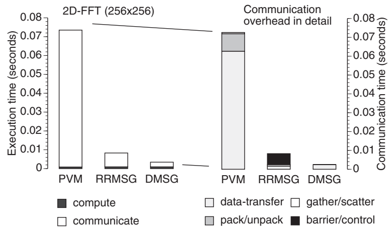
Figure 9.16: 2D-FFT ( 256 \times 256 ) for different message passing models: detailed breakdown of execution time [128 nodes].
