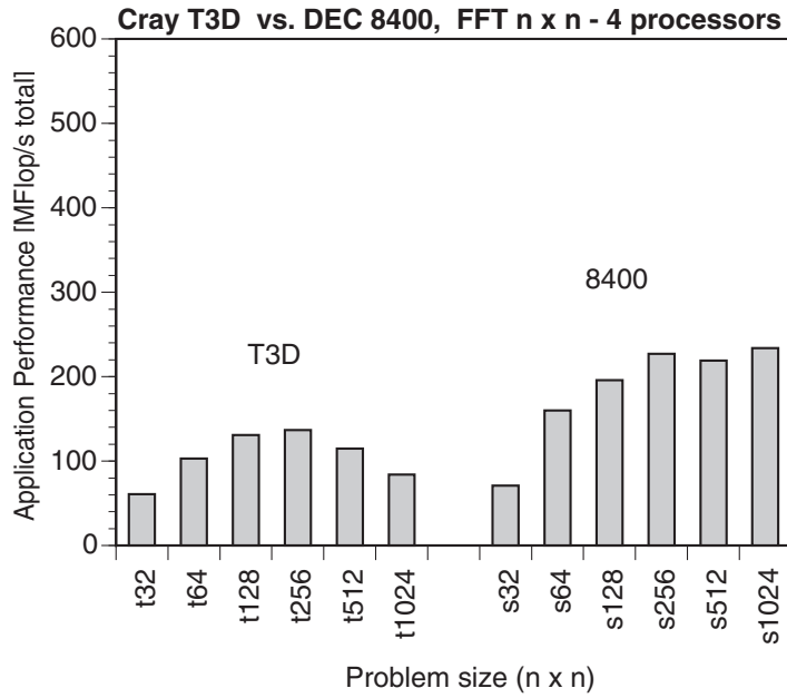
Figure 9.31: Total application performance of the 2D-FFT benchmark on 4 processors of a Cray T3D (left) and a DEC 8400 (right). Benchmark written in C.
