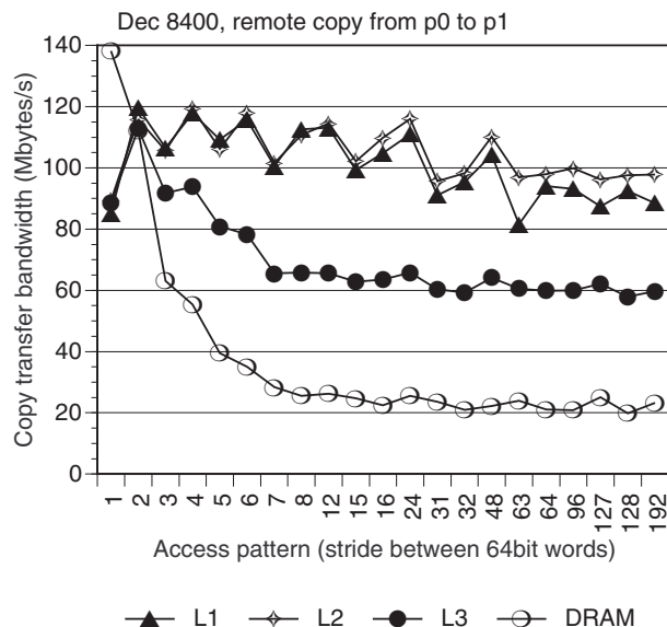
Figure 8.5: Measured performance of remote copy transfers between two processors (P0 and P1) of the DEC 8400 for different strides and for different characteristic working sets.
