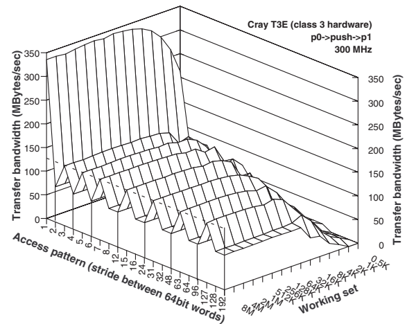
Figure 8.11: Cray T3E under deposit model: Transfer bandwidth for different access patterns (strides) and different working sets, obtained through remote stores.
