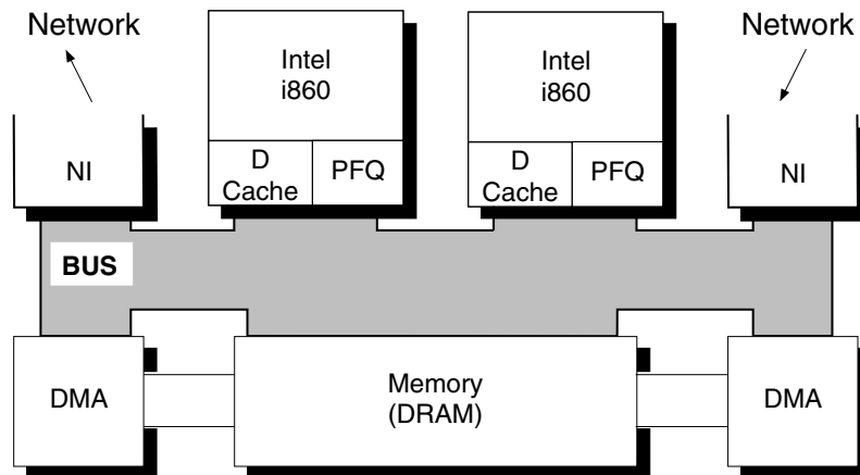
Figure 2.5: Overview of the Intel Paragon node architecture: NI refers to the network interface circuitry and with control logic and FIFOs for data transfers.
