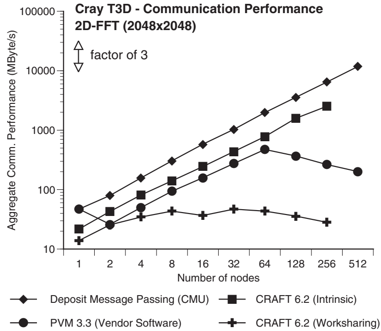
Figure 7.4: Aggregate communication performance of a 2048 \times 2048 point 2D-FFT for different machine sizes of Cray T3D, graphed on a log-log scale.
