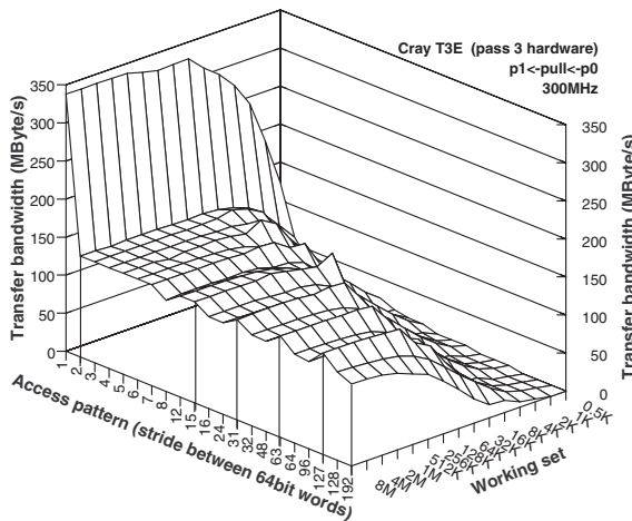
Figure 8.10: Cray T3E under fetch model: Transfer bandwidth for different access patterns (strides) and different working sets obtained through remote loads.
