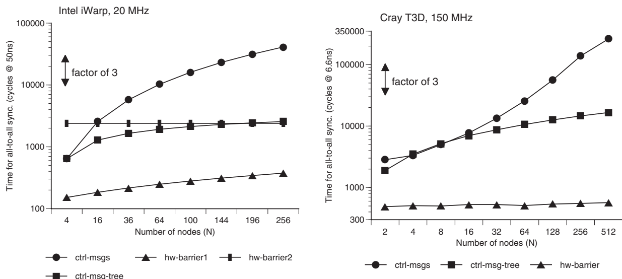
Figure 5.4: Costs of different mechanisms for control transfer (e.g. flow control) in an all-to-all communication step on iWarp and Cray T3D.
