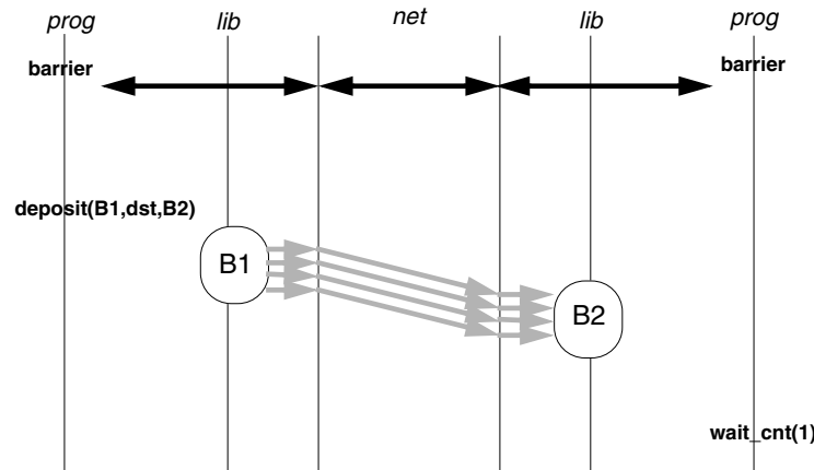
Figure 4.6: Expected communication behavior in the deposit model. The figure graphs the interactions between two processors along a wall clock time-line (top) to (bottom).
