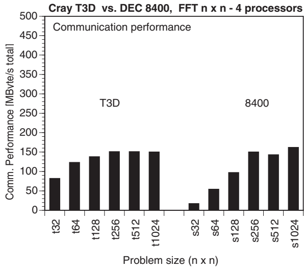
Figure 9.33: Communication performance in the transposes of the 2D-FFT benchmark on 4 processors of a Cray T3D and a DEC 8400. Compiler generated benchmark written in Fx Fortran (left) and hand-coded implementation in C (right).
