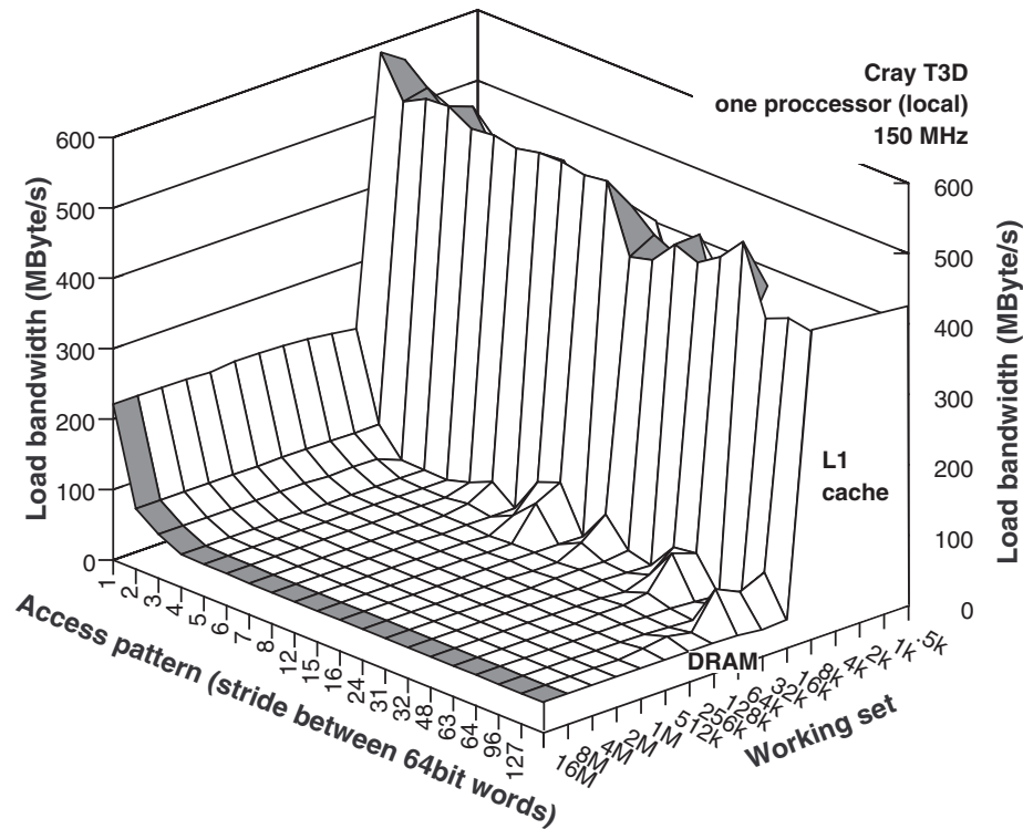
Figure 8.6: Cray T3D: Load bandwidth for different access patterns (strides) and different working sets. One processor runs memory benchmark, and the other three processors are idle.
