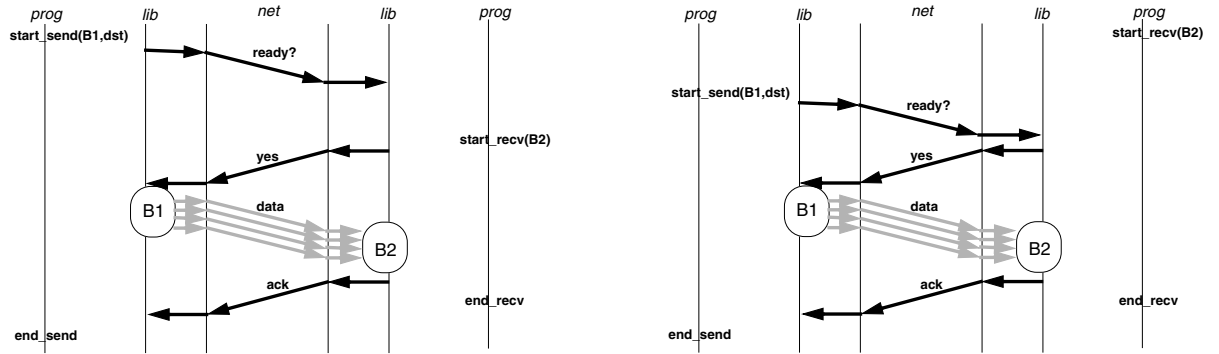
Figure 4.1: Expected communication behavior in the rendezvous model. Case when the sending processor enters first (left) and when the receiving processor enters first (right). The figure graphs interactions between two processors along a wall-clock time-line (top) to (bottom).
