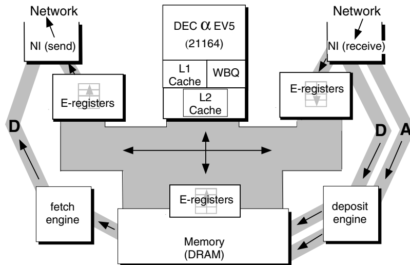
Figure 2.3: Overview of the Cray T3E node architecture: EREG refers to a block of fast registers in the support circuitry outside the microprocessor. NI refers to the network interface circuitry and with control logic and FIFOs for data transfers..
