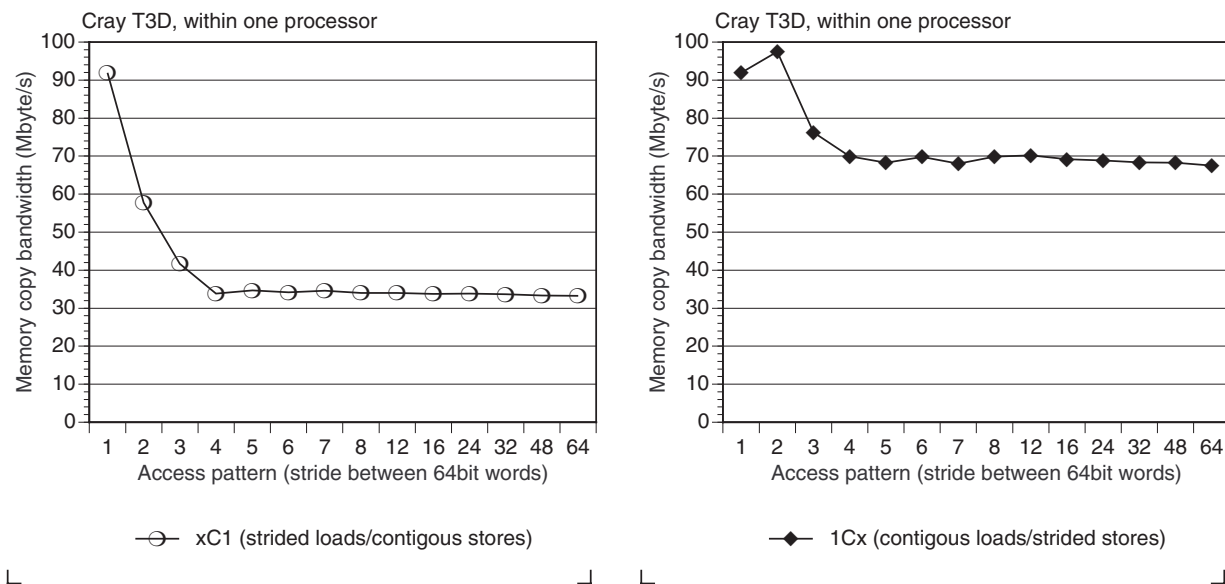
Figure 6.3: Measured performance of the local memory system for large transfer, with either strided loads or strided stores for the T3D.
