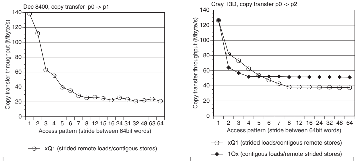
Figure 8.19: Measured performance of large remote copy transfers (i.e. between processors) on the DEC 8400 and the Cray T3D, for different strides.
