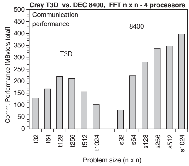
Figure 9.33: Communication performance in the transposes of the 2D-FFT benchmark on 4 processors of a Cray T3D and a DEC 8400. Compiler generated benchmark written in Fx Fortran (left) and hand-coded implementation in C (right).
