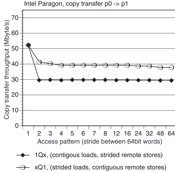
Figure 8.14: Measured performance of remote copy transfers between two processors (P0 and P1) of an Intel Paragon for different strides. Two options for strided accesses are considered, strides at the load end ( {}_xQ_1 ) and strides at the store end ( {}_1Q_x ).
