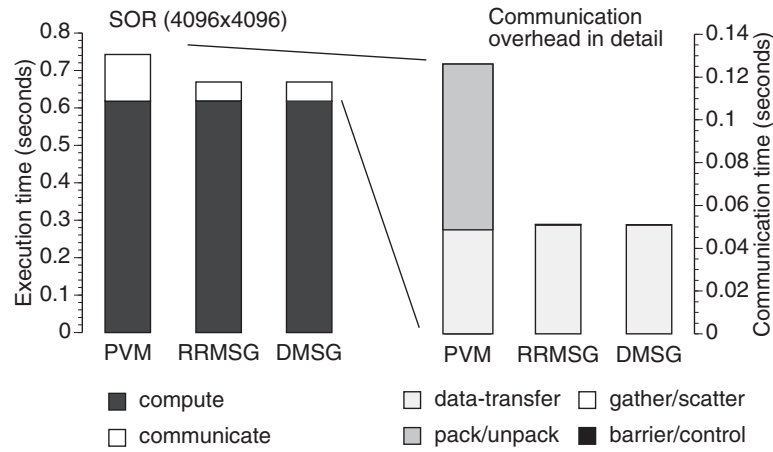
Figure 9.15: SOR ( 4096 \times 4096 ) for different message passing models: detailed breakdown of execution time [128 nodes].
