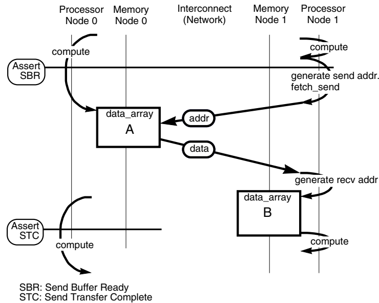
Figure 4.9: Control requirements and assertions in the of the fetch model.
