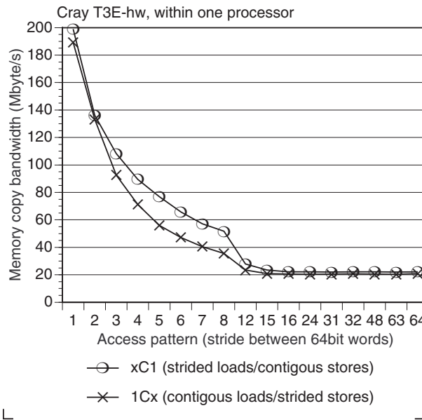
Figure 8.18: Measured performance of the local memory system for large transfers, with either strided loads or strided stores for the Cray T3E. Note the different scale.
