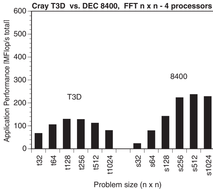
Figure 9.27: Total application performance of the 2D-FFT benchmark on 4 processors of a Cray T3D (left) and a DEC 8400 (right). Benchmark written in Fx Fortran.
