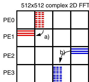
Figure 9.26: Execution of a 2D FFT includes an array transpose to change the distribution from row-major into column-major. Square patches must be moved between the processors. The patches of data can be moved in two ways, a) or b).
