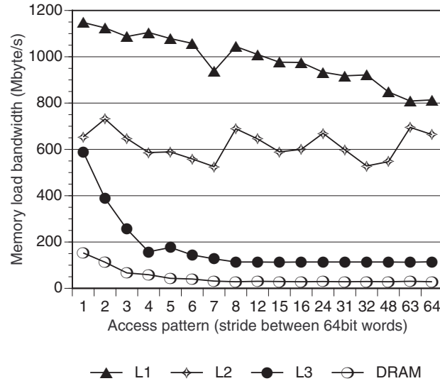
Figure 8.1: Bandwidth of loads for different access patterns (strides) and different working sets on the DEC 8400. One processor runs memory benchmark, other three processors are idle.
