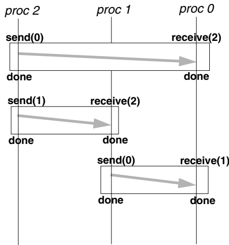
Figure 4.2: Example of a strongly synchronized program that executes correctly under the assumptions of the rendezvous model of message passing. The parameters of send/receive indicate the node i.e. send_to_node(1) and receive_from_node(2).
