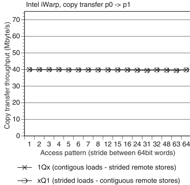
Figure 8.16: Measured performance of remote copy transfers between two processors (P0 and P1) of an Intel iWarp for different strides. Two options are considered for the access pattern, strides at the load end and strides at the store end.
