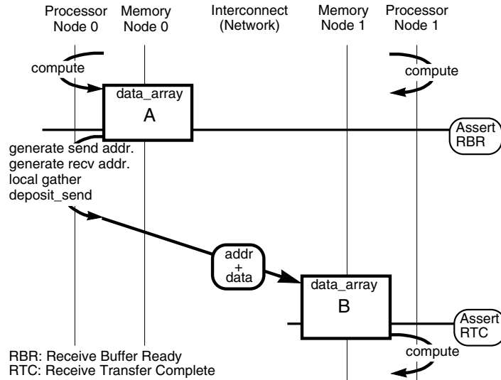
Figure 4.10: Control requirements and assertions in the of the deposit model.
