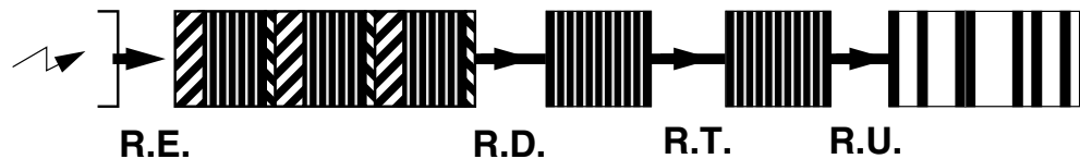
Figure 5.1: Potential copies of data elements as they occur in traditional message passing (e.g. PVM) due to coalescing of non-contiguous data transfers, protection domain crossing, and buffering to comply with synchronization semantics of postal model.
