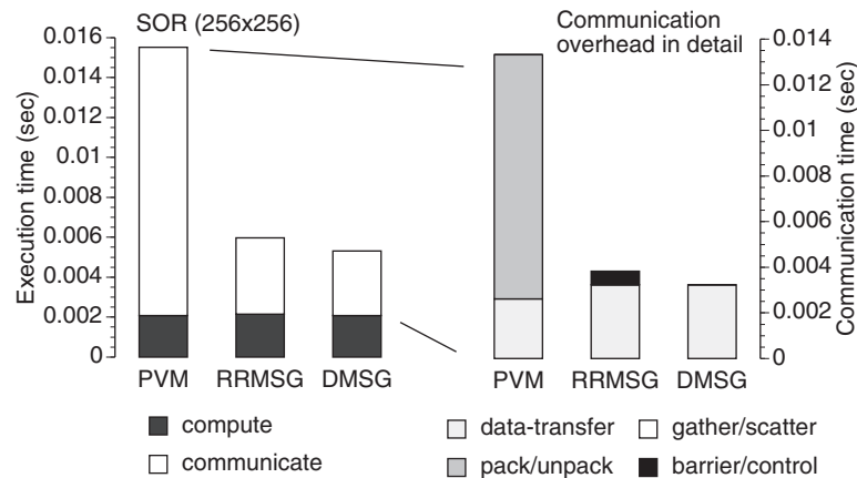
Figure 9.17: SOR ( 256 \times 256 ) for different message passing models: detailed breakdown of execution time [128 nodes].
