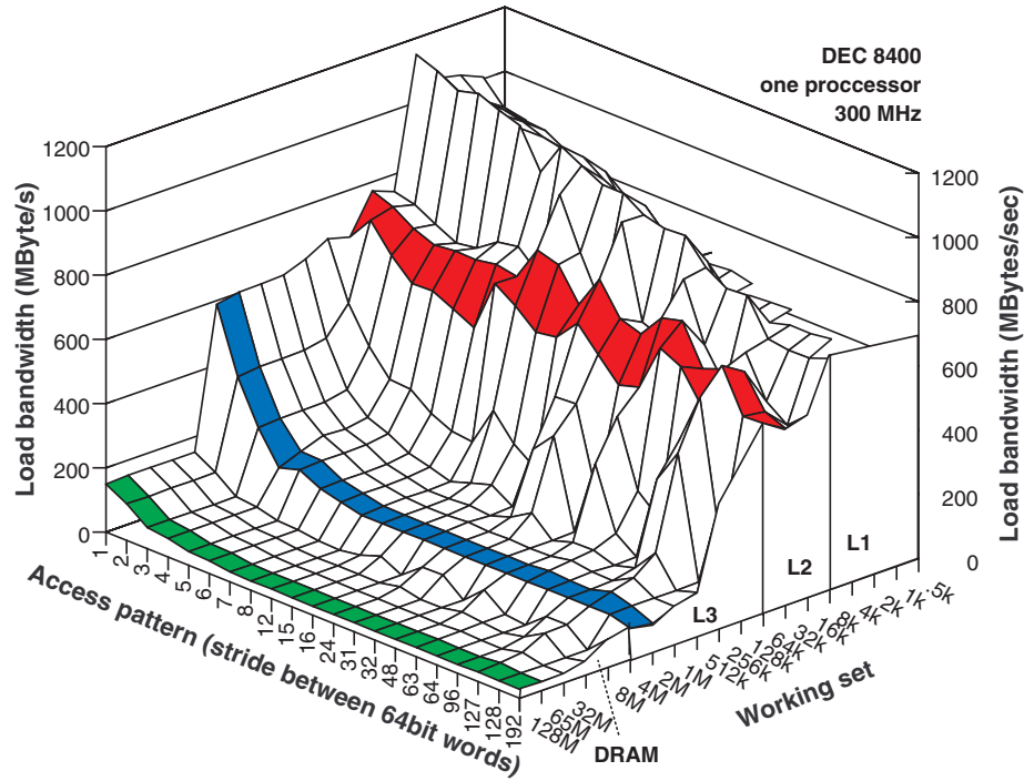
Figure 8.1: Bandwidth of loads for different access patterns (strides) and different working sets on the DEC 8400. One processor runs memory benchmark, other three processors are idle.
