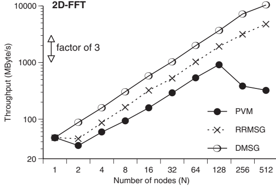
Figure 9.9: Aggregate communication performance of a 4096 \times 4096 point 2D-FFT, graphed on a log-log scale.
