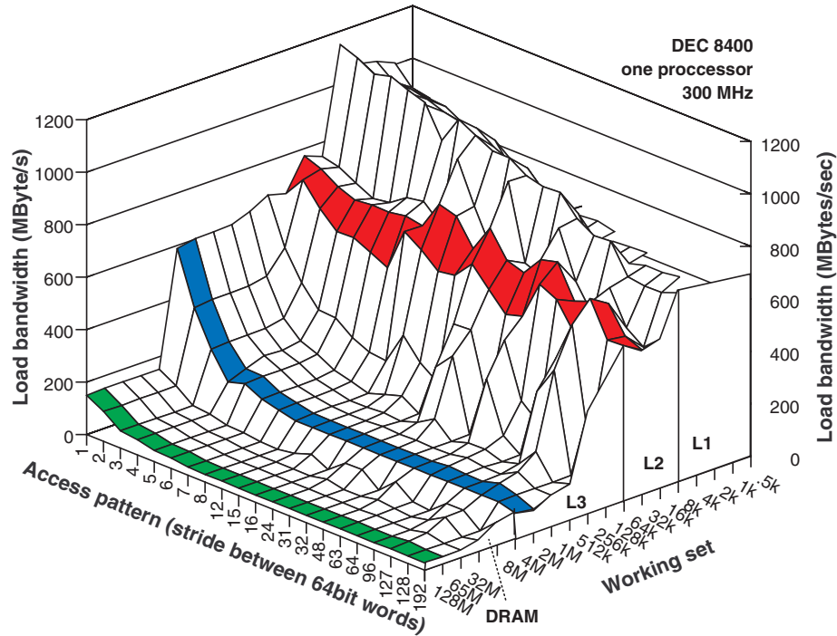
Figure 6.4: Bandwidth of loads for different access patterns (strides) and different working sets on a one processor DEC 8400.
