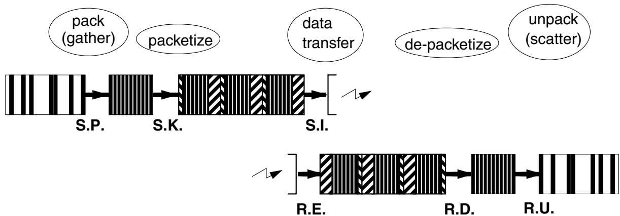
Figure 9.13: Possible copies of data occurring due to buffering for synchronization and coalescing of non-contiguous data transfers found in PVM a traditional message passing system.
