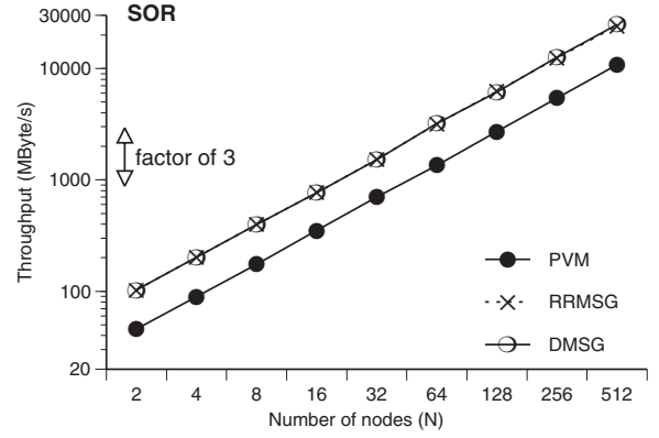
Figure 9.10: Aggregate communication performance of a 4096 \times 4096 element SOR, graphed on a log-log scale.
