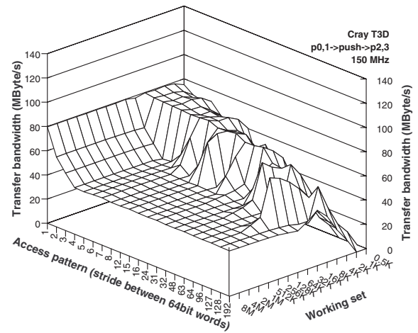
Figure 8.8: Cray T3D under deposit model: Transfer bandwidth for different access patterns (strides) and different working sets, obtained through remote stores.
