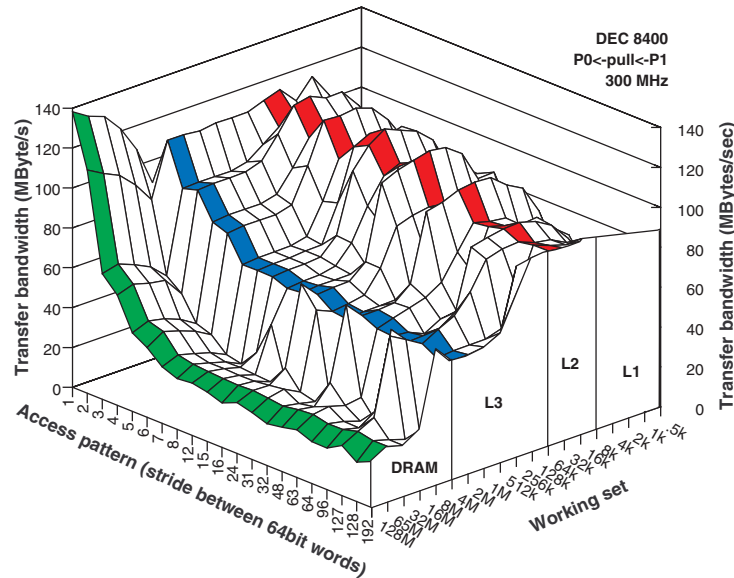
Figure 8.4: DEC 8400: Remote load bandwidth for different access patterns (strides) and different working sets. Throughput for transfers from processor P1 to processor P0.
