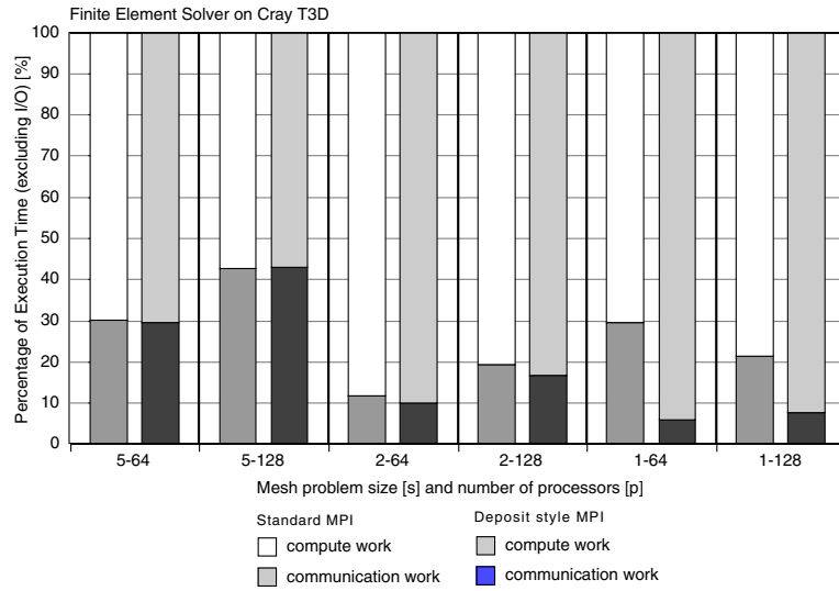
Figure 9.18: Fraction of execution time spent in communication for two MPI implementations of FEM (earthquake model) on a T3D. Left bar: a conventional postal message passing program and right bar: a deposit model program with split receives.
