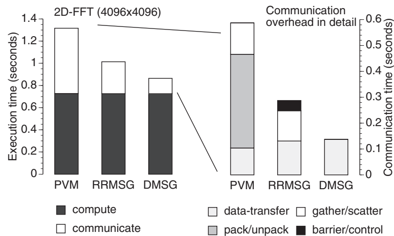
Figure 9.14: 2D-FFT ( 4096 \times 4096 ) for different message passing models: detailed breakdown of execution time [128 nodes].
