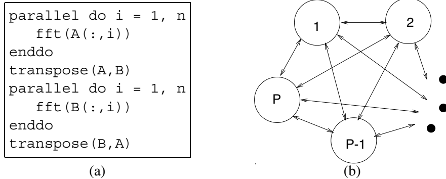
Figure 1.2: Basic operations of the 2D FFT program.
