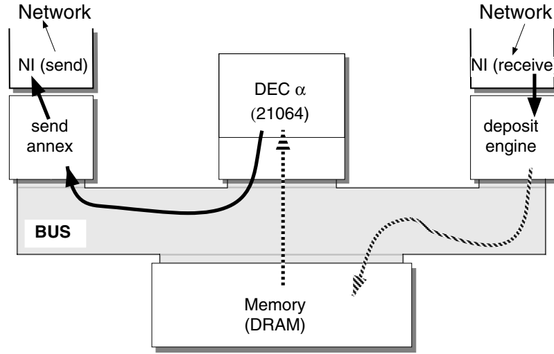
Figure 9.23: Schematic flow of data for chained communication in a Cray T3D node. Solid lines indicate streams of contiguous data, dashed lines potentially strided or indexed data.
