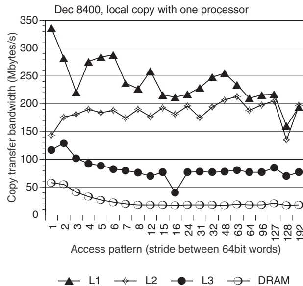
Figure 8.3: Measured local copy performance for strided loads on the DEC 8400 at four characteristic working sets.
