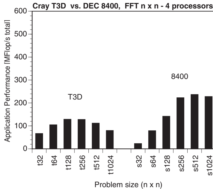
Figure 9.30: Total application performance of the 2D-FFT benchmark on 4 processors of a Cray T3D (left) and a DEC 8400 (right). Benchmark written in Fx Fortran.
