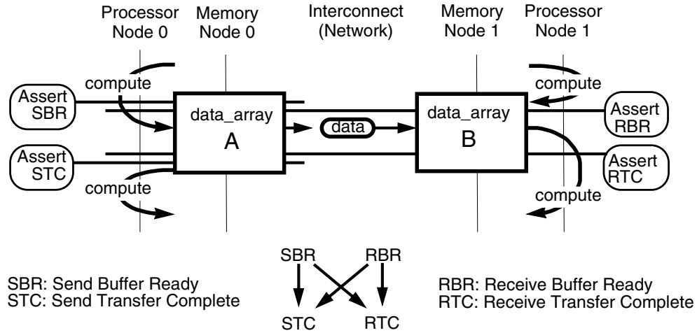
Figure 4.8: Control requirements and assertions in the of the rendezvous model.
