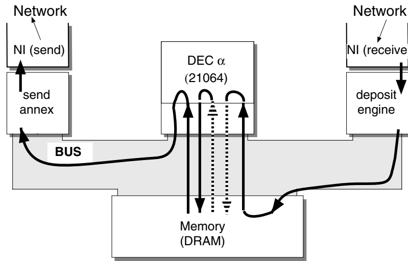
Figure 9.21: Schematic flow of data for buffer packing communication in a Cray T3D node. Solid lines indicate streams of contiguous data, dashed lines potentially strided or indexed data.
