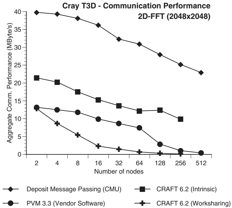
Figure 7.3: Per processor communication performance of a 2048 \times 2048 point 2D-FFT for different machine sizes of Cray T3D.
