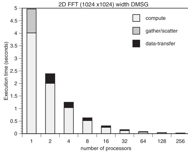
Figure 9.3: DMSG: Execution times of 2D-FFT for different Cray T3D machine sizes.
