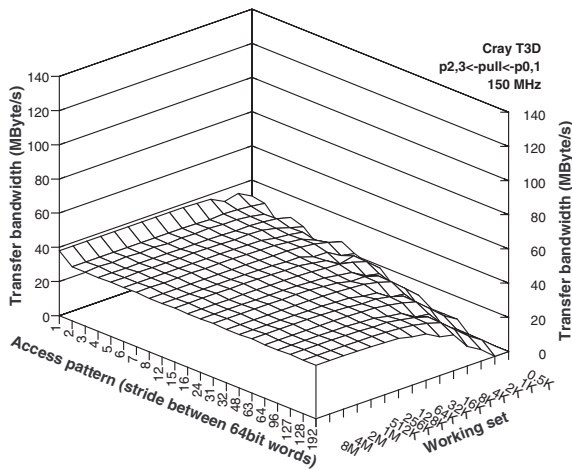
Figure 8.7: Cray T3D under fetch model: Transfer bandwidth for different access patterns (strides) and different working sets obtained through remote loads.
