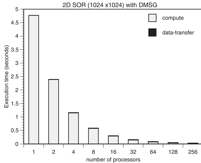
Figure 9.4: SOR: Execution times of 2D-FFT for different Cray T3D machine sizes.
