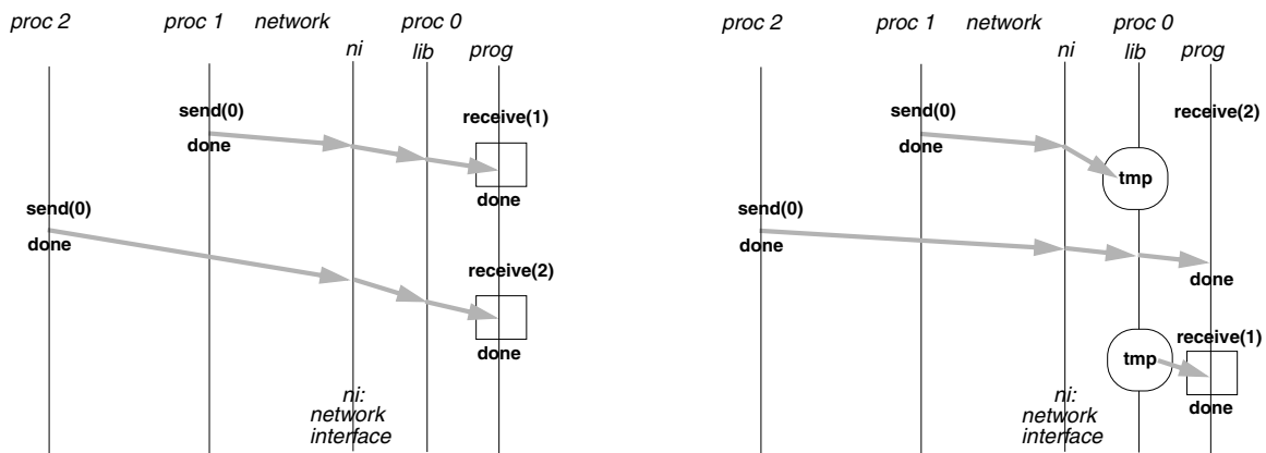
Figure 4.5: Example of a flow synchronized program that executes correctly under the assumptions of the postal model of message passing regardless of the timing and order of receive calls.
