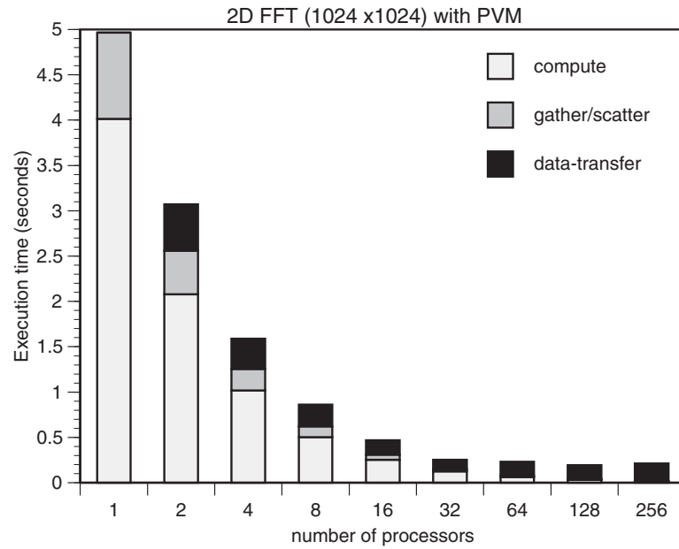
Figure 9.1: PVM: Execution times of 2D-FFT for different Cray T3D machine sizes.
