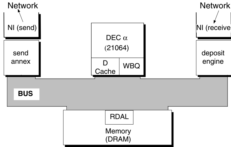
Figure 2.2: Overview of the Cray T3D node architecture: NI refers to the network interface circuitry and with control logic and FIFOs for data transfers.
