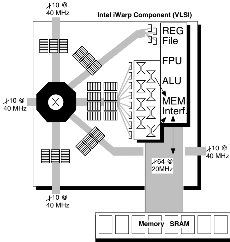
Figure 2.4: Overview of the Intel iWarp node architecture: The entire network interface is integrated into one single VLSI component.
