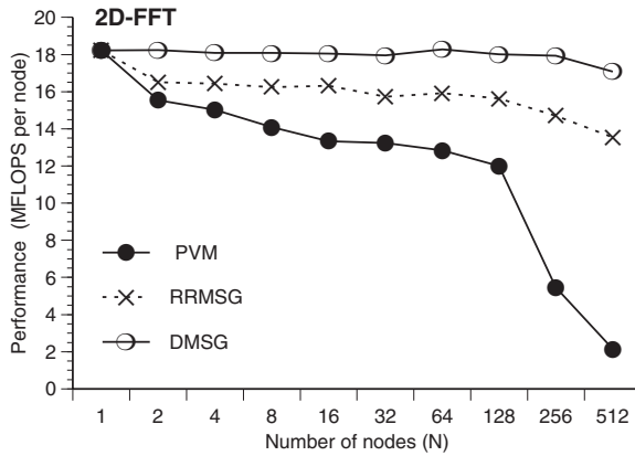
Figure 9.7: Per-node performance of a 4096 \times 4096 point 2D-FFT for different machine sizes.
