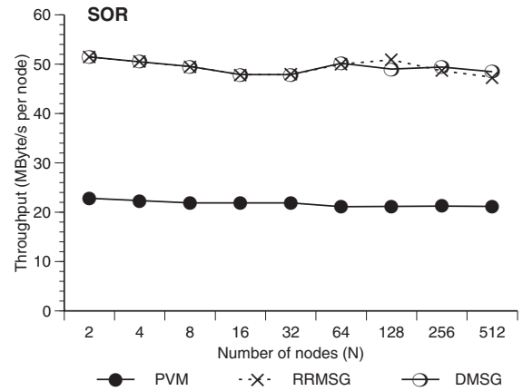
Figure 9.12: Per-node communication performance of a 4096 \times 4096 element SOR for different T3D machine sizes.
