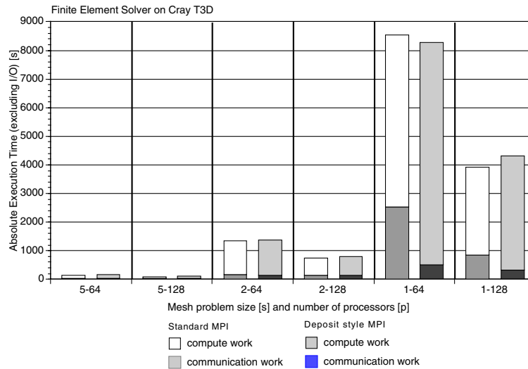
Figure 9.19: Execution times for two MPI implementations of FEM (earthquake model) on a T3D. Left bar: a conventional postal message passing program and right bar: a deposit model program with split receives.
