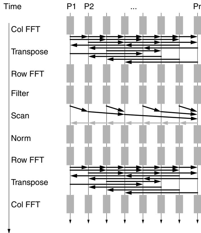
Figure 5.3: Computation and communications phases in typical applications.
