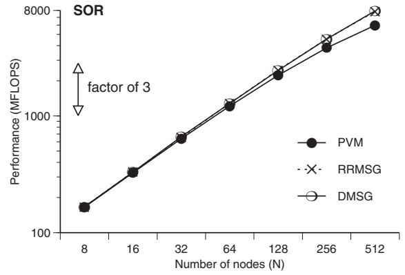
Figure 9.6: Aggregate performance of a 4096 \times 4096 element SOR for different machine sizes, graphed on a log-log scale.
