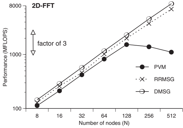
Figure 9.5: Aggregate performance of a 4096 \times 4096 point 2D-FFT for different machine sizes, graphed on a log-log scale.
