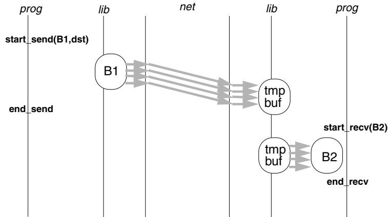
Figure 4.4: Expected communication behavior under the postal message passing model. The figure graphs the interactions between two processors on along a wall-clock time-line (top) to (bottom).
