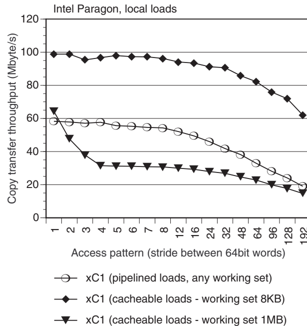
Figure 8.13: Intel Paragon: Load bandwidth for pipelined loads and cacheable loads for different access patterns (strides). The working set is large for pipelined loads, small and large cacheable loads.
