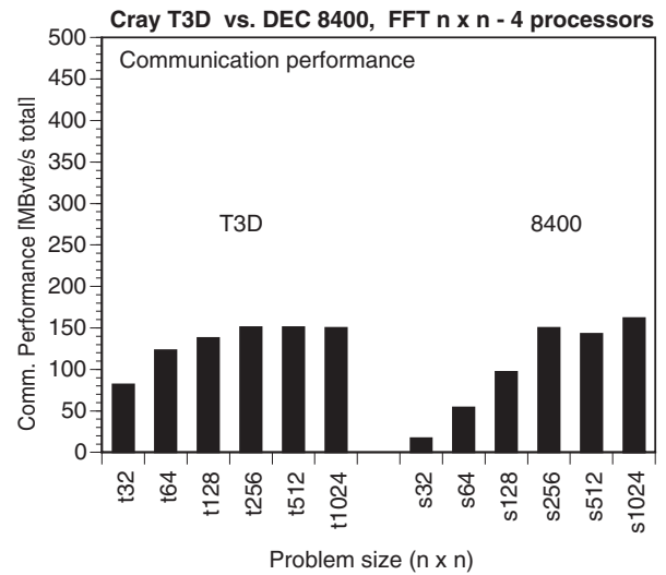
Figure 9.29: Communication performance in the transposes of the 2D-FFT benchmark on 4 processors of a Cray T3D (left) and a DEC 8400 (right). Benchmark written in Fx Fortran.
